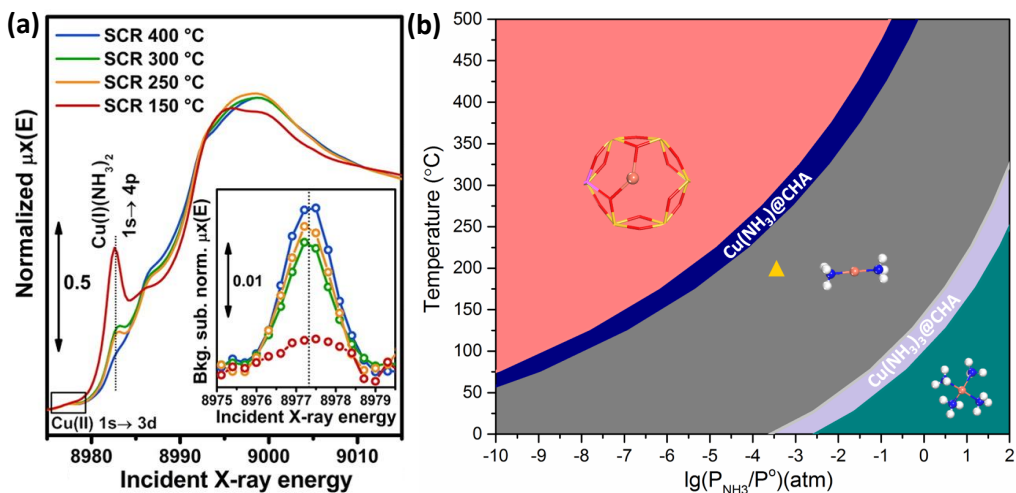
Figure 4.3: (a) Operando XANES spectra during \text{NH}_3 -SCR at 150, 250, 300 and 400 ^{\circ}\text{C} . (b) Phase diagram for \text{Cu}(\text{NH}_3)_x^+ in CHA with varying \text{NH}_3 pressure and temperature constructed from DFT. The yellow triangle indicates typical operating conditions, which corresponds to a temperature of 200 ^{\circ}\text{C} and an \text{NH}_3 concentration of 300 ppm. Atom color codes: copper (pink), aluminum (purple), nitrogen (blue), silicon (yellow), oxygen (red) and hydrogen (white). Figure (a) is reprinted with permissions from Ref. [113]. Copyright (2016) American Chemical Society.
