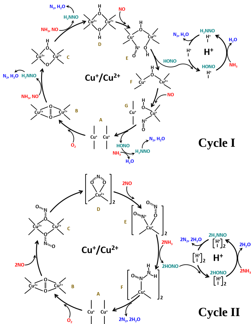
Figure 5.5: Two possible reaction cycles (Cycle I and II) for low-temperature \text{NH}_3 -SCR over Cu-CHA. Each cycle contains reaction intermediates on the \text{Cu}^+/\text{Cu}^{2+} sites and on the \text{H}^+ site. Dangling sticks connected to the Cu ions indicate the \text{NH}_3 ligands. The reactants, the reaction intermediates and the products are indicated in red, green and blue, respectively.
