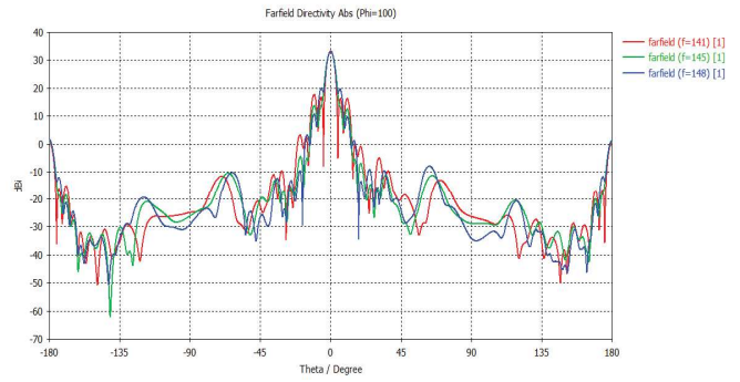
Fig. 4. The simulated H-plane radiation patterns at 141, 145 and 148 GHz.
