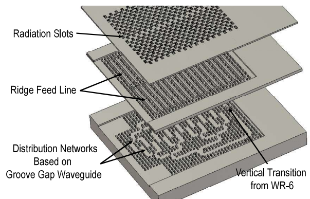
Fig. 1. Configuration of series-fed array antenna.
