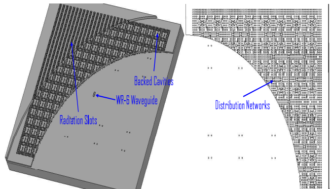
Fig. 6. Configuration of corporate-fed array antenna.
