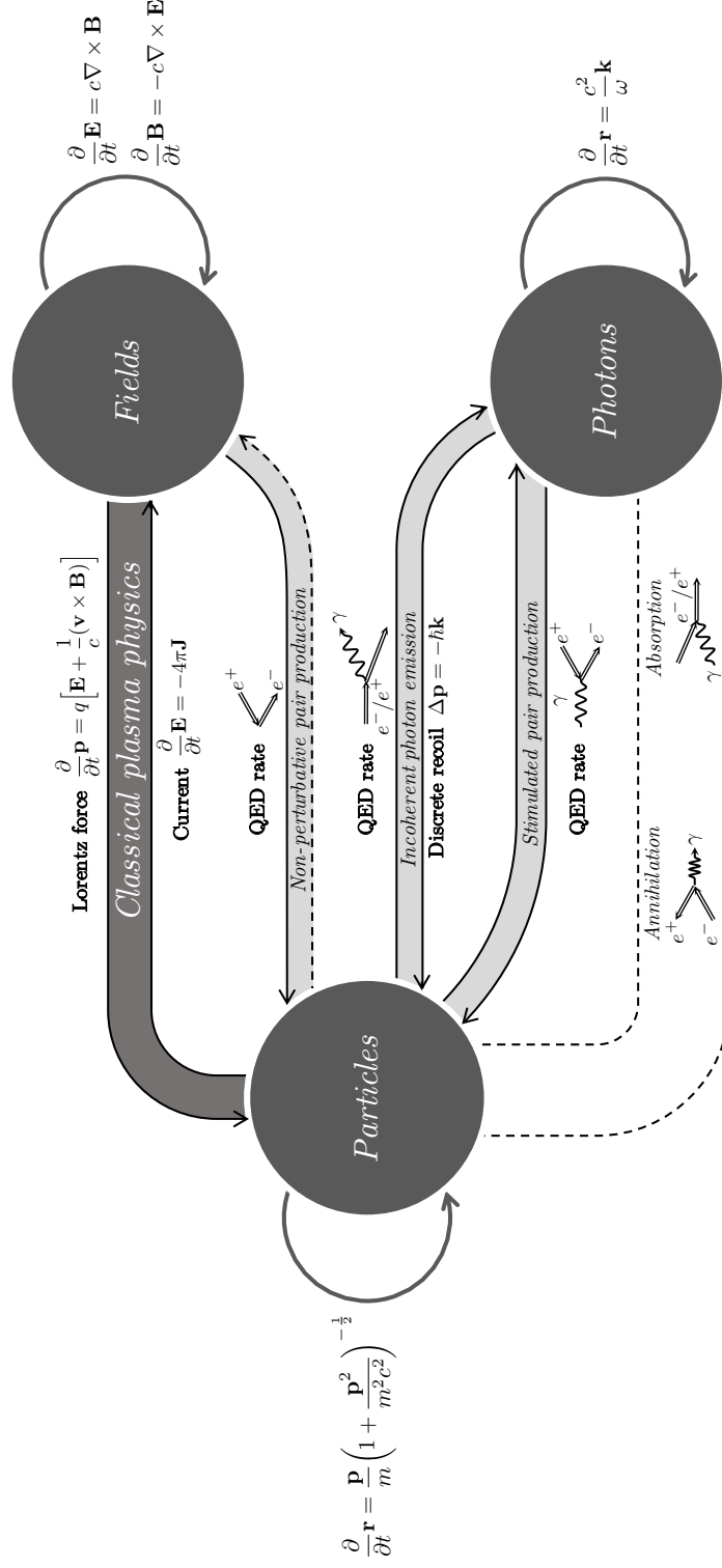
Figure 7.4: Diagrammatic representation of the QED-PIC scheme where the coherent radiation is represented by the fields and the incoherent radiation by photons . The figure has been adapted from Ref. [167].
