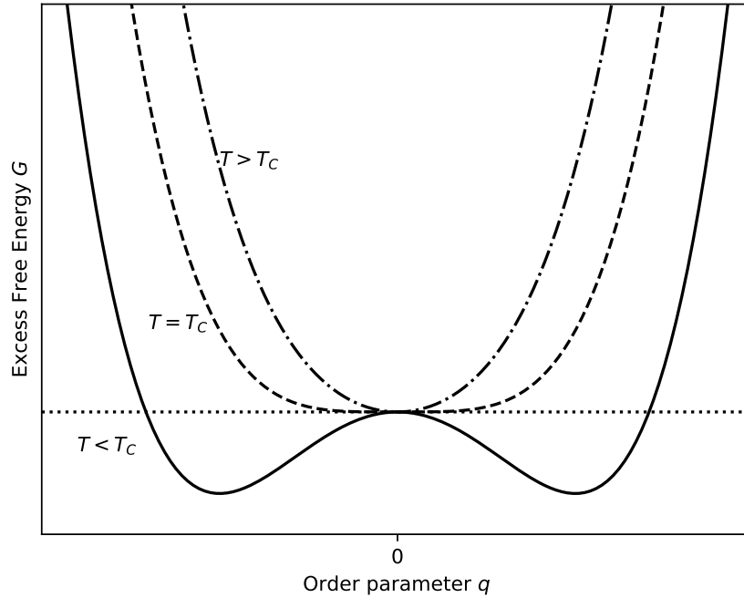
Figure 7.2: Schematic of the excess free energy as a function of the order parameter q at different temperatures T .
