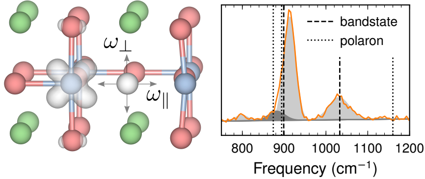
Figure 9.1: Close up of the measured INS spectrum in the interval 700–1250 \text{cm}^{-1} . Frequencies calculated with HSE are marked with dashed (bandstate) and dotted (polaron) lines. Gaussian fits are indicated by shaded areas.
