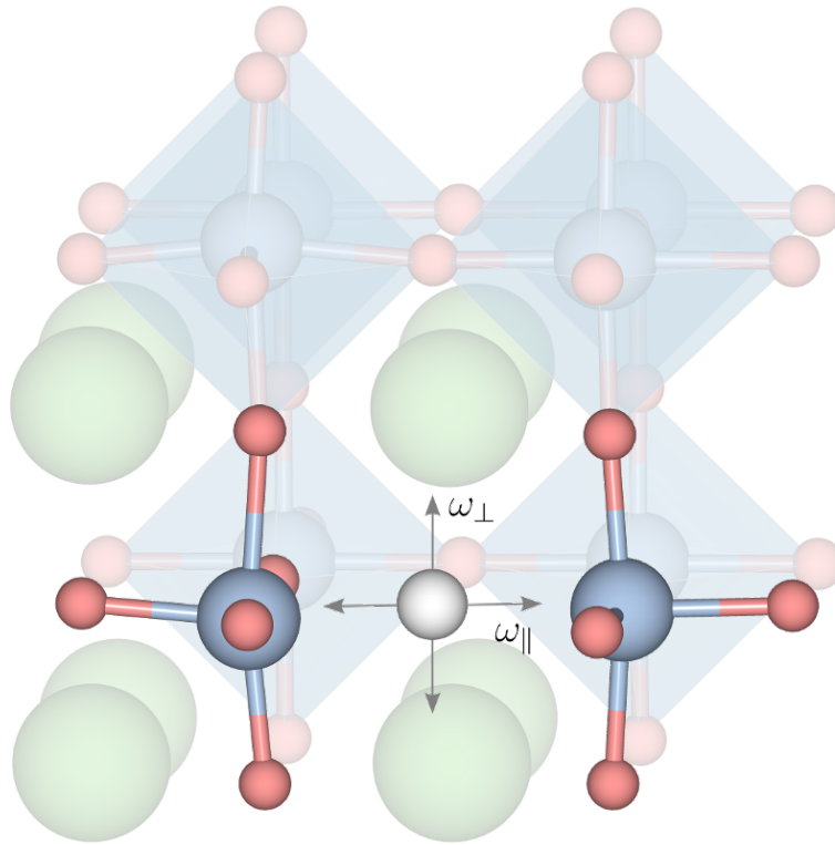
Figure 5.3: Illustration of hydride vibrational modes in the oxyhydride BaTiO 3 .
