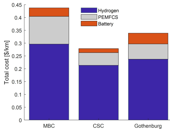
Fig. 14: Comparative result among MBC, CSC, and Gothenburg cycle.
