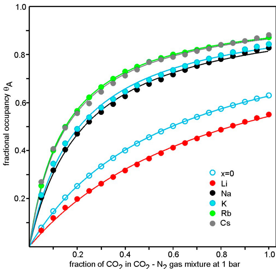
Figure 8. Adsorption isotherms from TGA data for A_{2/3}\text{Cu}[\text{Fe}(\text{CN})_6]_{2/3} compounds and \text{Cu}[\text{Fe}(\text{CN})_6]_{2/3} ( x = 0 ). The temperatures were 20 \pm 1 °C. The solid lines are fits to the Langmuir expression \theta_A = V/V_m = K_{eq} \cdot p_A / (1 + K_{eq} \cdot p_A) .
