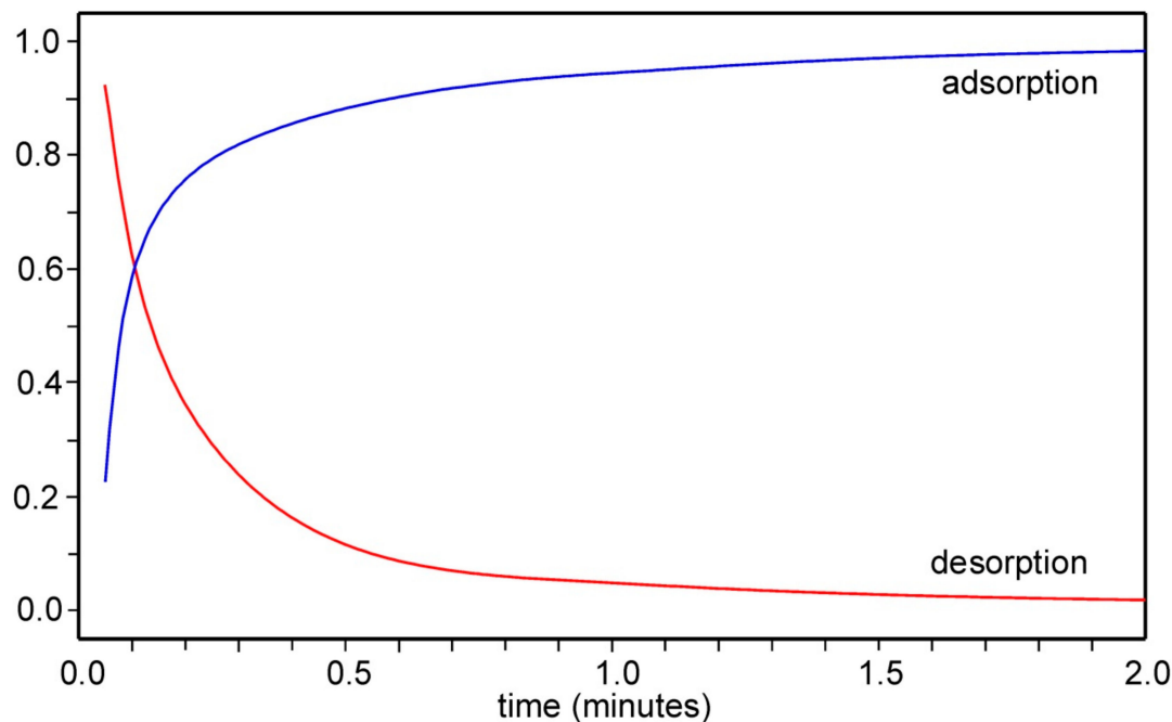
Figure 9. Curves showing normalised TGA adsorption and desorption steps of \text{CO}_2 on nominal \text{Li}_{2/3}\text{Cu}[\text{Fe}(\text{CN})_6]_{2/3} at 21\text{ }^\circ\text{C} . The sample weight was ~16 mg.
