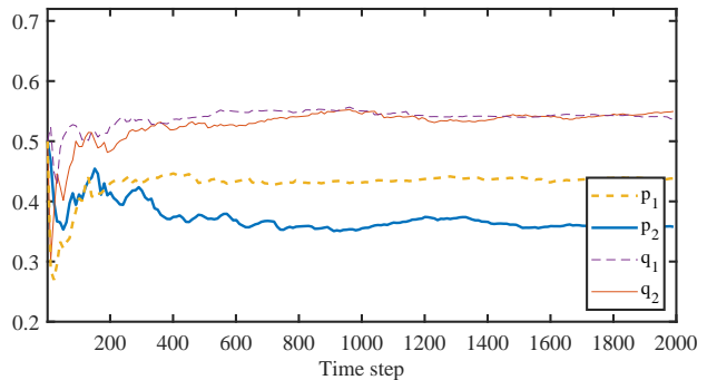
Fig. 6. Performance of the algorithm in learning the unknown parameters when a marginally stable ( i \in \{1\} ) and an unstable ( i \in \{2\} ) subsystem compete for a single communication channel. The channel quality is assumed to be similar for all subsystems with p = 0.3 and q = 0.6 .
