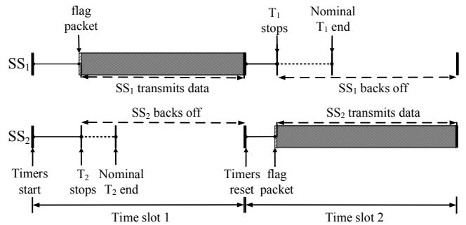
Fig. 3. Example of 2 subsystems competing for one channel in 2 successive time slots. Subsystem 1 (denoted as SS_1 ) has the largest cost in the first time slot and gets the access to the channel. Subsequently, subsystem 2 (denoted as SS_2 ), that did not communicate in the first time slot, in the second time slot gets to have a larger cost. Here, m_{2,1,2} > m_{1,1,2} and thus SS_2 gets access to the channel.
