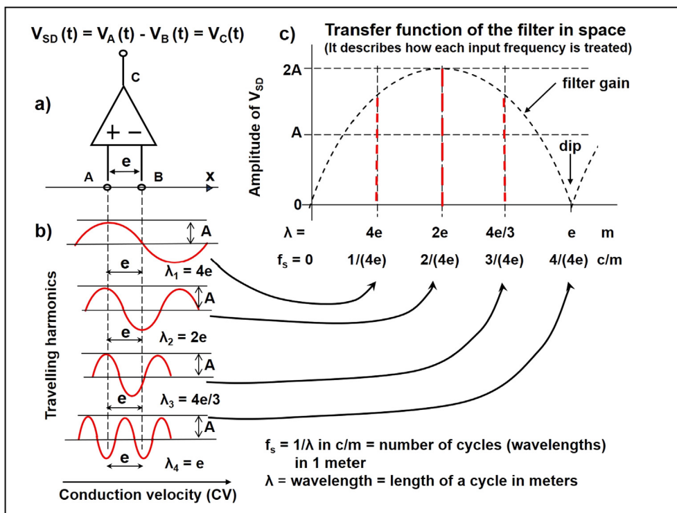
Fig. 13. Spatial filtering effect of a differential detection system. (a) Differential detection system, (b) four harmonics of the spatial signal distribution moving along with velocity u . (c) Amplitudes of the four harmonics observed in point C ( V_{SD} ).
