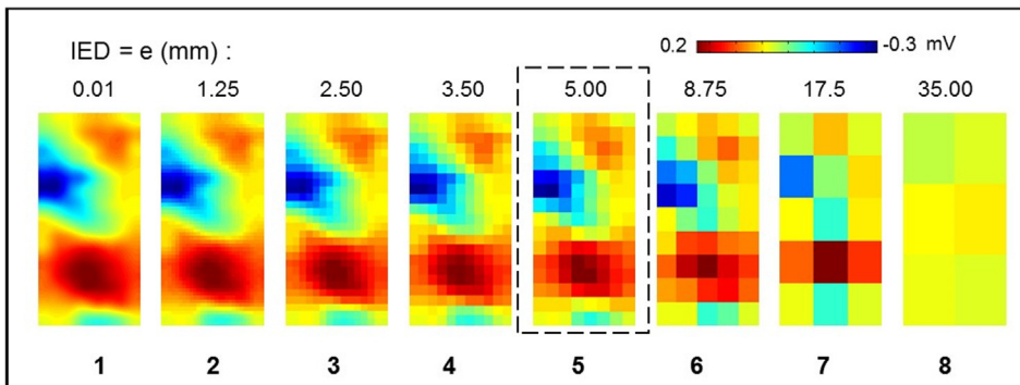
Fig. 15. sEMG image interpolation. Image 5 is the spatially sampled version ( e = 5 mm, electrode diameter = 1 mm) of an analog sEMG frame from a biceps brachii muscle. Image 1 is the result of interpolation with a “sinc” function and can be considered as the reconstructed analog image. All the other images (2–8) are obtained by resampling image 1 in space. Images 1 to 4 can still be reconstructed by interpolation of image 6 but not from images 7 and 8. Image size: 35 \times 70 mm. Courtesy of S. Soedirdjo.
