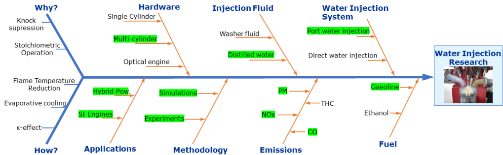
Figure 1.10: An Ishikawa (fish-bone) diagram representing various sections and fields of water injection research in SI engines
