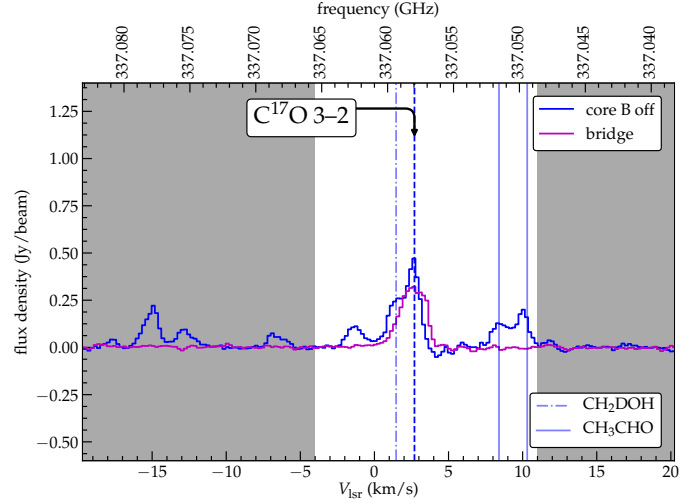
Fig. A.1. Spectral profiles of C 17 O 3–2 at two spatial positions: one beam west-southwest of source B (blue “×” mark in Fig. 2) and within the bridge filament (magenta “+” mark in the same figure). The frequency of the species of interest is marked by the blue, vertical dashed line; other lines identified in the frequency range are marked with dotted, dash-dotted, or solid lines. All rest frequencies are shifted by +2.7 km s −1 to account for the systemic velocity of source B. The section of the velocity axis with white background denotes the maximum range over which intensities are integrated.
