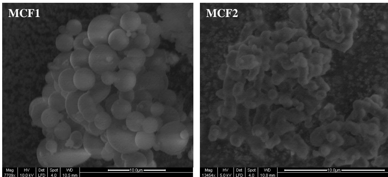
Figure 25. Representative SEM image of MCF1 and MCF 2.
