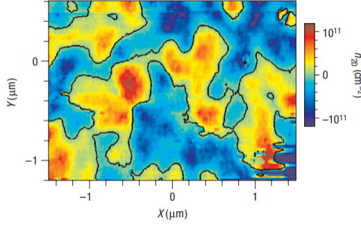
Figure 2.4: Charge carrier density profile measured at the Dirac point [40].
