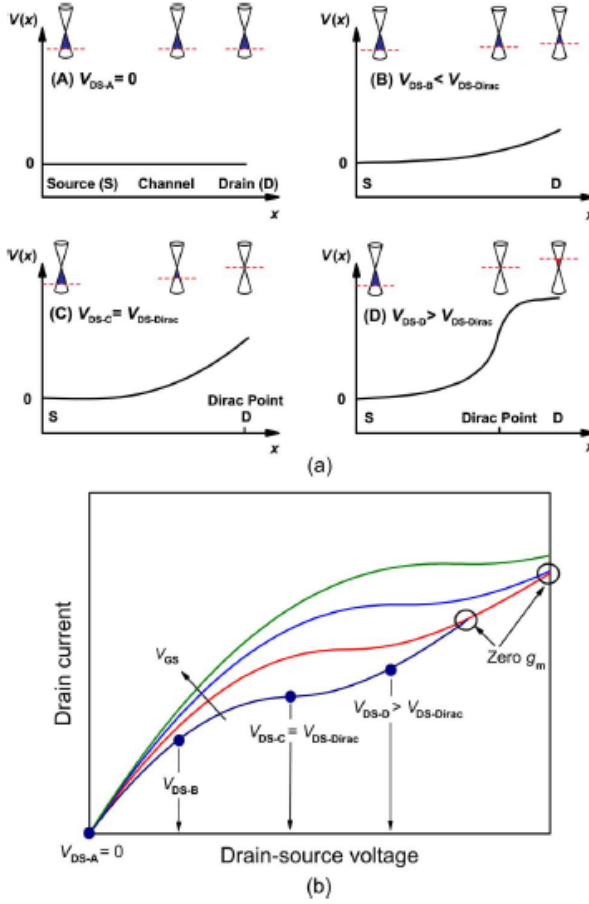
Figure 4.2: (a) shows the potential profile along the channel in GFET for four different drain-to-source biases ( V_{ds} ) (b) output characteristic shows the behaviour of drain current corresponding to four different V_{ds} biases and similar behaviour of drain current for different gate-source ( V_{GS} ) voltage [6, 57].
