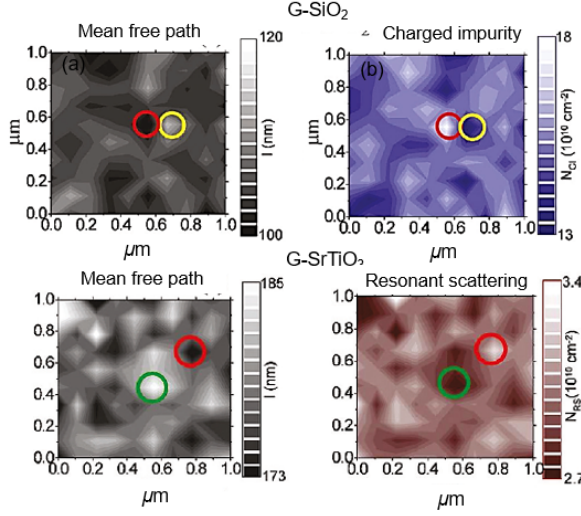
Figure 2.5: (a) Map of mean free path of electrons in graphene on \text{SiO}_2 (b) in relation with 2D spatial distributed charged impurities map (c) map of mean free path of electrons in graphene on \text{SrTiO}_3 and (d) corresponding map of the density of resonant scattering centers [35].
