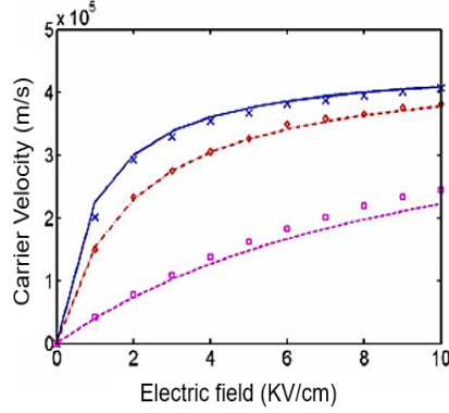
Figure 4.7: The charge carrier velocity vs the applied electric field as a function of different impurity concentration decreases from top to bottom. The crosses (×) correspond to no impurity and the squares (□) represents highest impurities [101].
