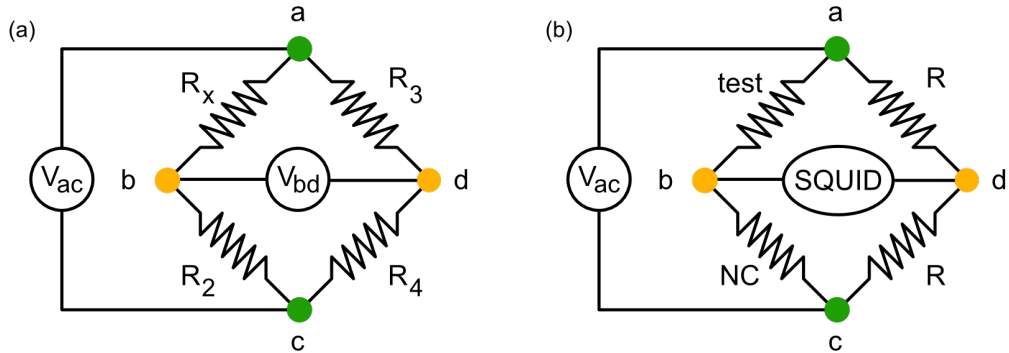
Figure 4.4: (a) A Wheatstone bridge circuit. This circuit is used to either measure an unknown resistor or changes in a known resistor, R_x , using two balanced arms of resistors. The voltage is applied between points a and c and the adjusting resistor R_2 is used to null the voltage drop across points b and d. The unknown resistor can thus be calculated: R_x = \frac{R_2 \times R_3}{R_4} . (b) Equivalent circuit of the Wheatstone bridge for the differential ac magnetic susceptibility measurement setup.
