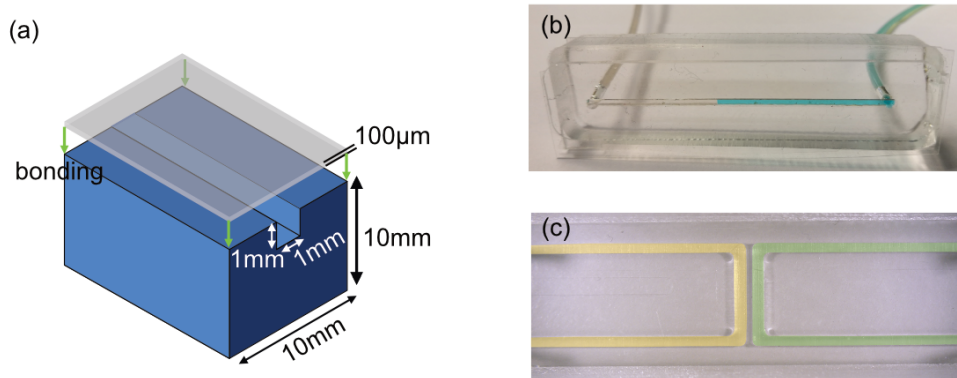
Figure 3.11: (a) The dimensions of the microfluidic channel, and photographs of completed (b) single channel, and (c) double-channel PDMS chips enclosed by bonding a 100 \mu\text{m} thin PDMS cap layer.
