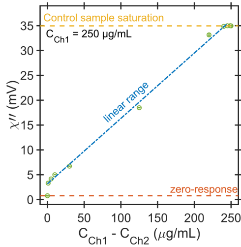
Figure 3.16: The amplitude of the imaginary component of the differential ac susceptibility peak at 100 Hz versus the difference in the concentration of MNPs in the two channels. When the difference in the two concentrations is large, the background magnetic signal makes it difficult to distinguish small differences in the test sample, and the imaginary susceptibility saturates to that of the control sample signal amplitude. The blue line indicates the linear range of operation and has a regression coefficient of 0.99 (excluding the zero-response and the saturation values). Adapted from paper III.
