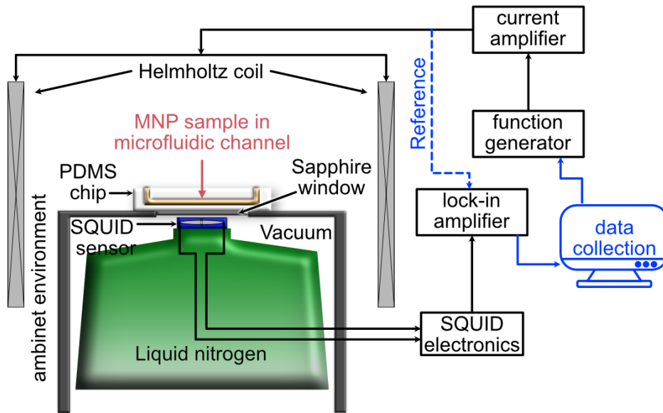
Figure 3.4: A schematic diagram of the lock-in measurement setup and a cross-section schematic illustration of the LN 2 cryostat for magnetic ac susceptibility measurements. The function generator through a current amplifier drives the Helmholtz coil to produce homogeneous ac magnetic excitation field. The SQUID readout signal from the SQUID electronics and a reference signal at excitation frequency, which is a voltage drop across a small resistor ( 0.01\Omega ) placed in line with the Helmholtz coil, are given to the lock-in amplifier for phase sensitive measurement. The in-phase and out-of-phase components of the signal are collected by a computer using a program interface in MATLAB ver. R2018b (The MathWorks, Inc., Natick, Massachusetts, United States).
