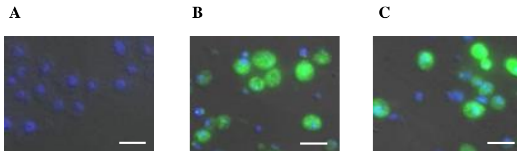
Figure 24: Cellular localization of ATP7B. Immunostaining of ATP7B variants in yeast cells using a ATP7B-specific antibody. All nuclei were visualized by DAPI staining. \Delta ccc2\Delta atx1 yeast A. without any ATP7B plasmid as control, B. with wild type ATP7B, or C. with M3H2A ATP7B variant high-copy plasmid. (Scale bars 5 \mu m).
