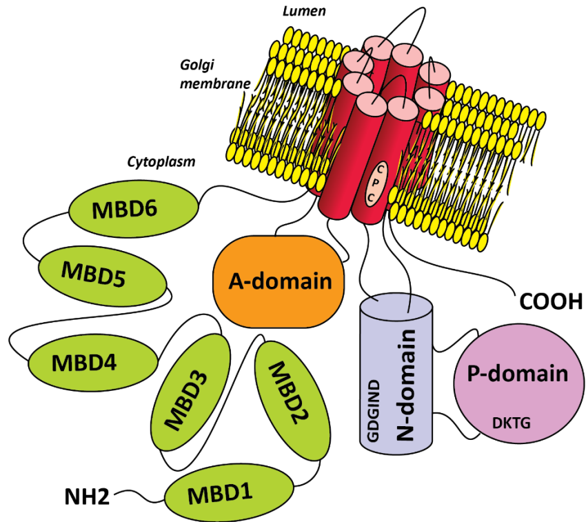
Figure 6: Structural organization of ATP7B. Domains of a Cu-P 1B type ATPase is illustrated for ATP7B; TMDs (red), six MBDs (green), A-domain (orange), P-domain (pink) and N-domain (blue, HP locus is present in this region). The linker that connects MBD4 and MBD5 consists of 76 residues which is the longest among other linkers. The linker between MBD3-MBD4 is 29 residues long, between MBD2-MBD3 is 24 residues in length, between MBD1-MBD2 is 13 residues and 6 residues between MBD5-MBD6 in ATP7B
