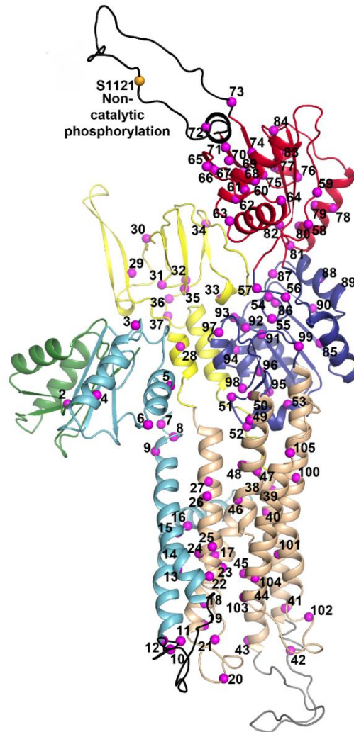
Figure 7: Three dimensional model of ATP7B. Homology model of ATP7B (1-4 \Delta MBD). The TMD (helices) are connected to MBD6 (cyan). MBD5 (green), A-domain (yellow), P-domain (blue), and N-domain (red). Magenta spheres indicate missense WD mutations (Gourdon et al. 2012). Used by permission of De gruyter, from Gourdon (2012).
