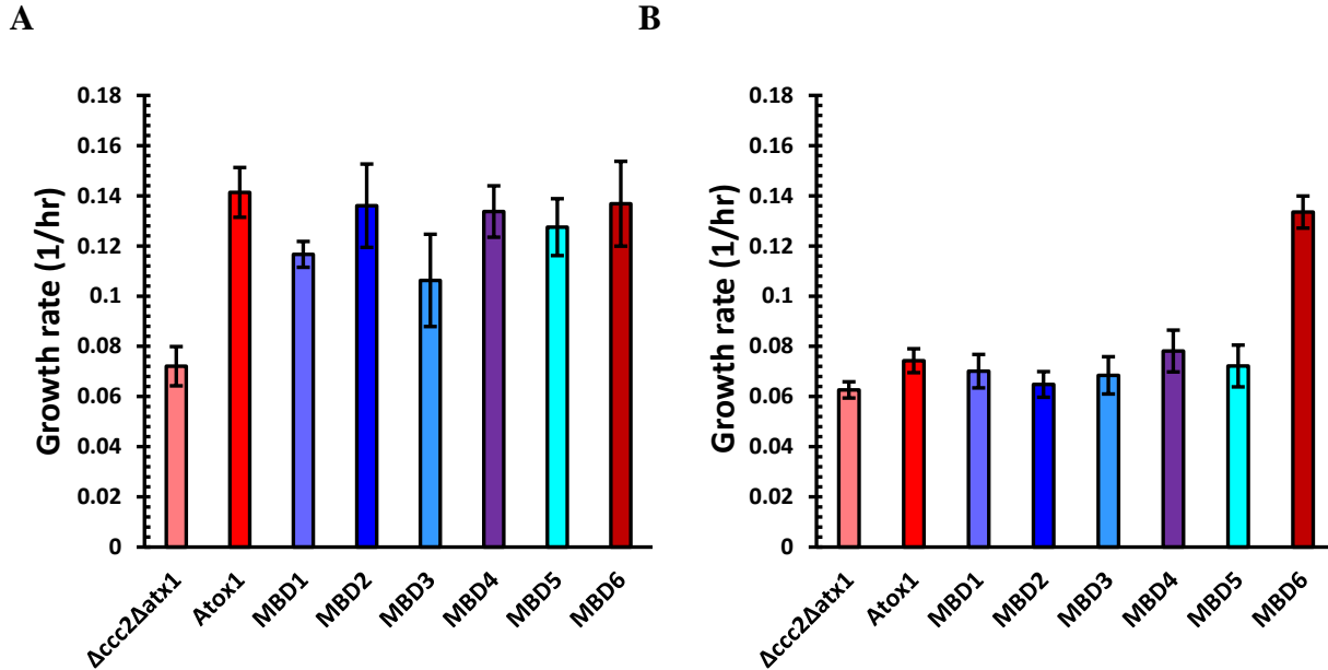
Figure 20: Growth rates of yeast expressing individual MBDs instead of Atox1, along with domain-truncated ATP7B variants in the Accc2Δatx1 yeast strain at Fe-limited conditions. A. Individual MBDs and full-length ATP7B. B. Individual MBDs and ATP7B DEL1-6. Error bars are based on standard deviations calculated for quadruplicate experiments.
