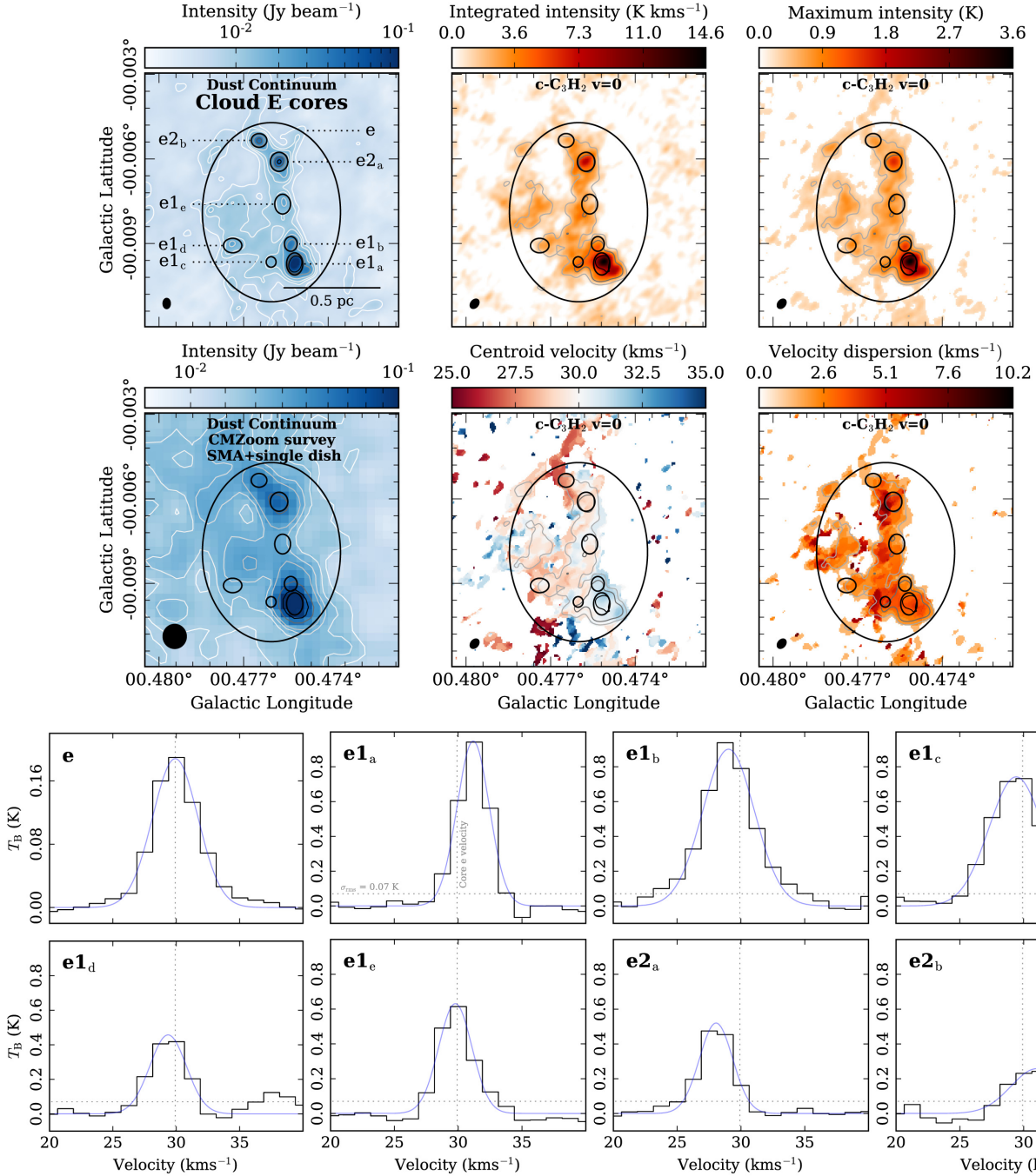
Figure 8. Upper two rows: Dust continuum (measured with ALMA and the SMA) and moment maps of the c\text{-C}_3\text{H}_2 v=0 7(0,7) - 6(1,6) transition towards the Cloud E/F proto-cluster region (as labelled in each panel). Overlaid on upper row left-hand panel are the ALMA continuum contours of [10, 15, 20, 30, 50, 70, 90] \sigma_{\text{rms}} , where \sigma_{\text{rms}} \sim 0.6 mJy beam ^{-1} . Overlaid on the second row left-hand panel are SMA continuum image are contours of [3, 4, 5, 6, 9, 12] \sigma_{\text{rms}} , where \sigma_{\text{rms}} \sim 7 mJy beam ^{-1} . Overlaid on the remaining map panels are maximum intensity contours of [0.21, 0.42, 0.63, 0.84, 1.05, 1.4, 2.1] K. All contours increase in colours from white to grey to black. Labelled are the individual cores e1_a , e1_b , e1_c , e1_d , e1_e , e2_a , e2_b that have been identified within this region, and the average region covering all these cores, referred to as the proto-cluster (region e ). Lower two rows: The average spectra of the c\text{-C}_3\text{H}_2 v=0 7(0,7) - 6(1,6) transition taken from each of the regions. For reference, overlaid on each spectrum are vertical and horizontal dotted lines, which show the systemic velocity of the proto-cluster region, and the \sigma_{\text{rms}} level of \sim 0.07 K. Also shown are the profiles of the Gaussian fits to each spectrum (fit parameters are given in Table 5).
