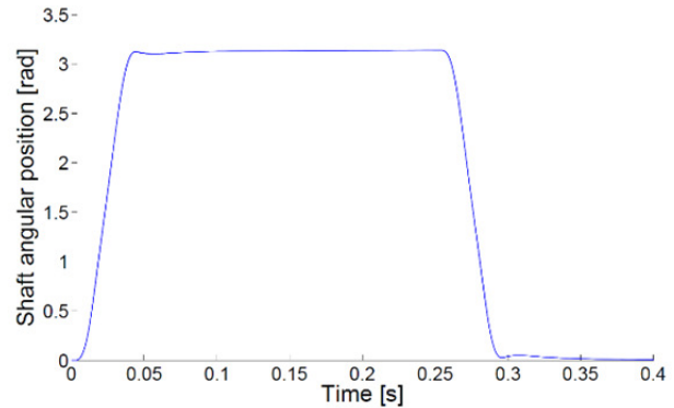
Figure 4: Shaft position with 6 superimposed scan cycles.
