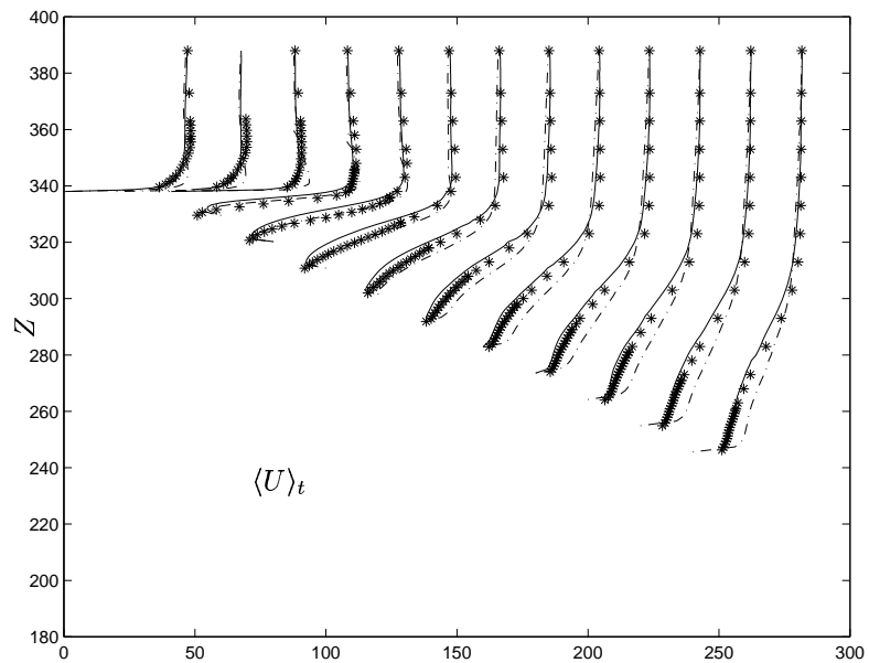
Figure 10: Time-averaged streamwise velocity profiles in the symmetry plane. Medium grid (solid curve); coarse grid (dashed-dotted curve); experiment (symbols).
