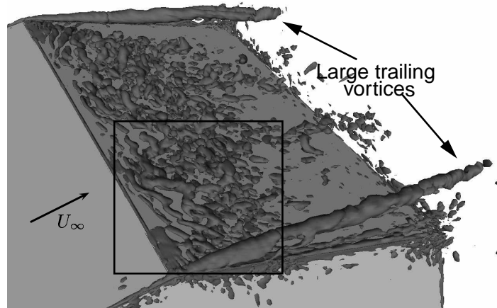
Figure 3: The isosurface of the instantaneous second invariant of the velocity gradient, Q = 3000 . The direction of the flow is from left to right. Note that only the rear slant surface is shown.
