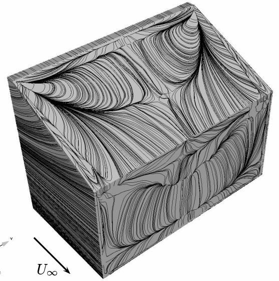
Figure 7: Comparison of a) oil-film visualization by Lienhart and Becker [7] at Re = 7.68 \times 10^5 with b) time-averaged trace lines on the surface of the body from LES. Only the rear part of the body is shown. View from behind the body.
