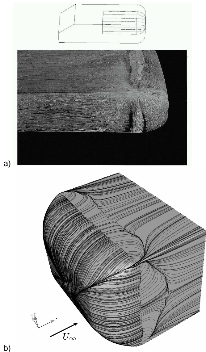
Figure 5: Comparison of a) oil-film visualization by Sims-Williams and Dominy [4] at Re = 1.71 \times 10^5 with b) time-averaged trace lines on the surface of the body from LES. Flow is from right to left in Fig. a) and from left to right in Fig b).
