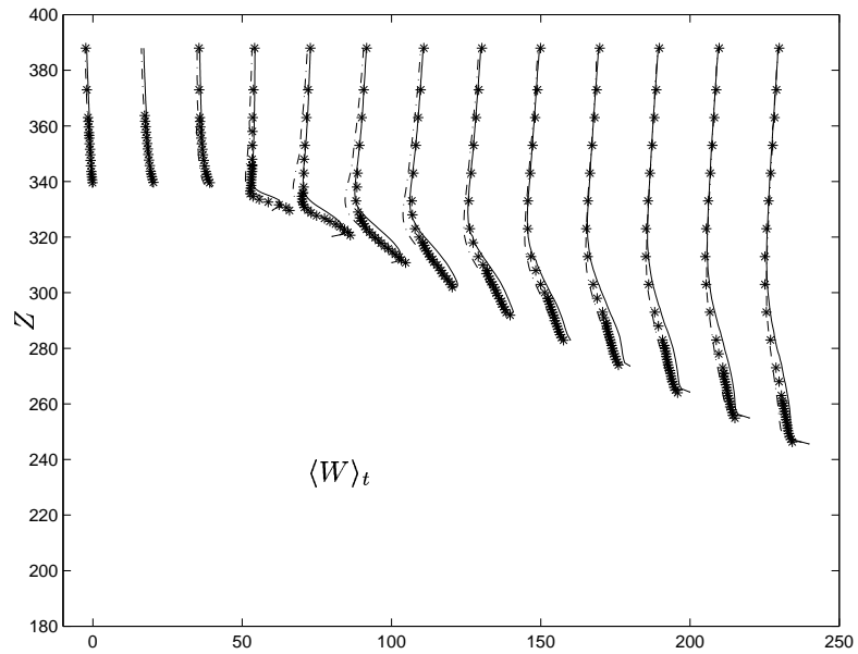
Figure 9: Time-averaged wall-normal velocity profiles in the symmetry plane. Medium grid (solid curve); coarse grid (dashed-dotted curve); experiment (symbols).
