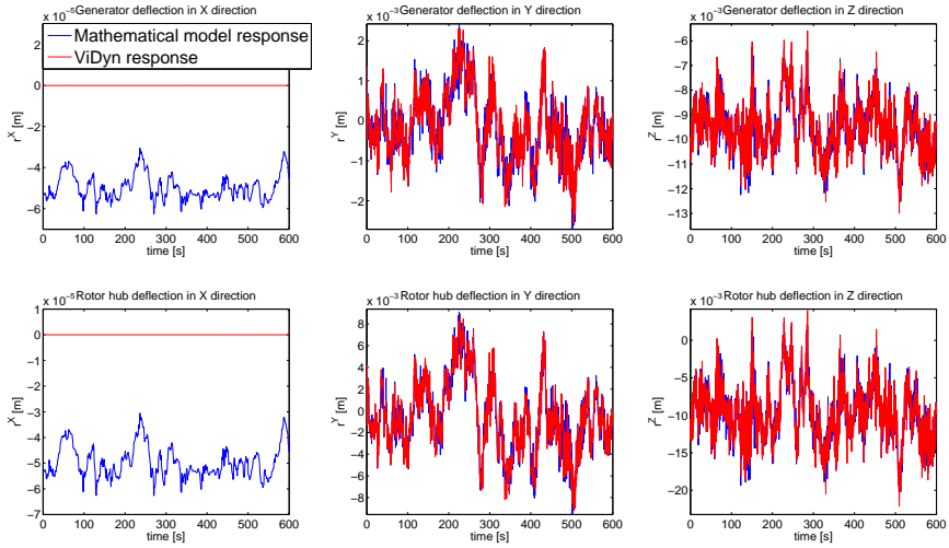
Fig. 8 The deflection fields at generator (up) and rotor hub (down), in OS^2 (11 m/s), Math — blue —, and ViDyn — red — models
