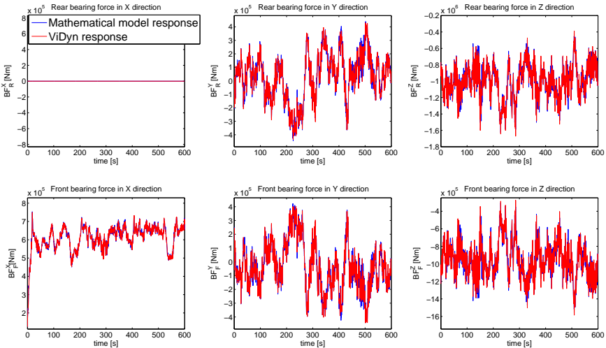
Fig. 9 The bearing forces in rear (up) and front (down), in OS^2 (11 m/s), Math — blue —, and ViDyn — red — models
