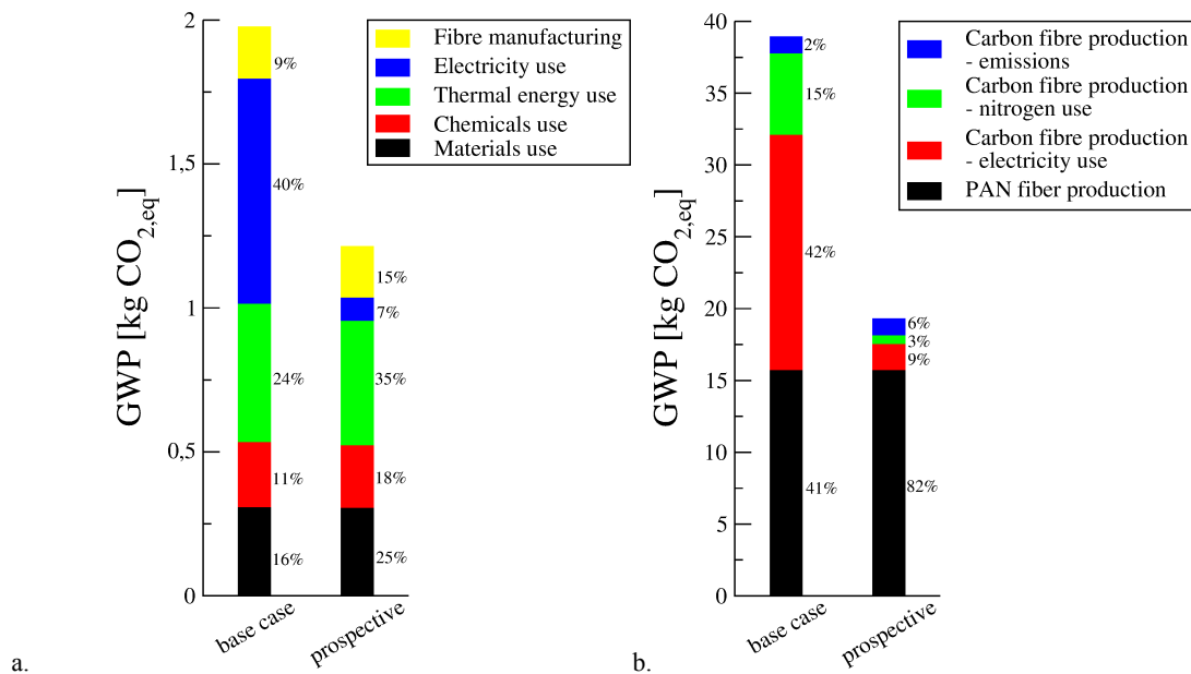
Figure 5: Climate impact (measured using global warming potential (GWP)) to produce: a. 1 kg of glass fibre and b. 1 kg of poly-acrylonitrile-based carbon fibre, for the base case and prospective production systems.
