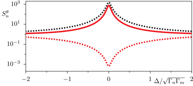
FIG. 24. Linear squeezing spectra S_n^\theta(\Delta) vs. input detuning for two-mode squeezing under non-degenerate and degenerate resonance 39,46 . Non-degenerate resonance (red solid); degenerate resonance, \theta = -\pi/4 (black dashed) and \theta = \pi/4 (red dashed). The amplification (squeezing) is localized in small detuning interval, \Delta \ll \Gamma_j at large gain. [ \epsilon = 0.95\sqrt{\Gamma_n\Gamma_m} , \delta = 0 , \Gamma_m = 3\Gamma_n , \Gamma_n = \Gamma_{n0} .]
