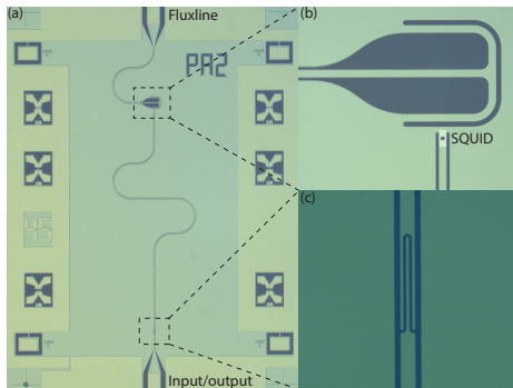
FIG. 1. Micrographs of a typical tunable resonator: (a) full chip (5x7 mm) with the flux line at the top, and the input/output port with the coupling capacitor at the bottom; (b) SQUID together with the inductive coupling between the flux line and the SQUID loop; (c) Coupling capacitor. (Adopted from 38 , courtesy of A. Bengtsson.)
