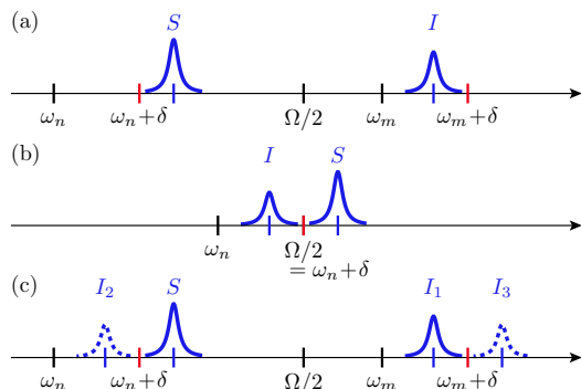
FIG. 5. Mode structure of amplified output field for a detuned input signal (S), for (a) the two-mode amplification of (a) non-degenerate parametric resonance and (b) degenerate parametric resonance, and for (c) the four-mode amplification. Black color indicates cavity resonances, red color marks parametrically coupled strong field modes; solid blue lines indicate signal (S) and (primary) idler ( I_1 ) with frequencies, \omega_n + \delta + \Delta and \omega_m + \delta - \Delta ; dashed blue lines indicate secondary idlers ( I_{2,3} ) with frequencies, \omega_n + \delta - \Delta and \omega_m + \delta + \Delta .
