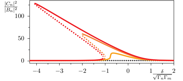
FIG. 8. Nonlinear gain |C_n|^2/|B_n|^2 vs pump detuning \delta , for the non-degenerate parametric amplifier and on-resonance input, \Delta = 0 , with \epsilon_n/\Gamma_n = 0.8, 0.9, 0.95 (from bottom to top); black dotted line refers to the Duffing limit \epsilon_n = 0 . [ |B_n|^2 = 2\Gamma_n , \theta_B = 0 , B_m = 0 , \alpha_n/\Gamma_n = 0.01 , \alpha_n = \alpha_m , \Gamma_n = \Gamma_m .]
