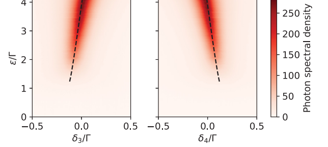
FIG. 17. Nondegenerate parametric oscillations of modes n = 3 and n = 4 observed experimentally 67 emerge at finite detuning from the resonance, \omega_j + \delta , and exhibit frequency drift with increasing pumping intensity, in accord with the theory, Eqs. (54) and (55).
