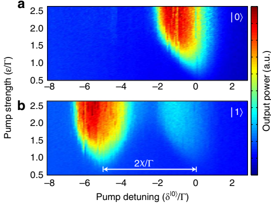
FIG. 16. Output radiation of parametrically pumped cavity with dispersively coupled qubit, for the ground state (a) and excited state (b) of the qubit, 2\chi is a dispersive shift produced by the qubit; the low intensity spot in panel (b) is due to qubit relaxation during measurement 77 .
