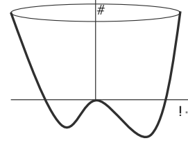
FIG. 19. Tilted metapotential of the degenerate oscillator, cut along optimum phase direction.
