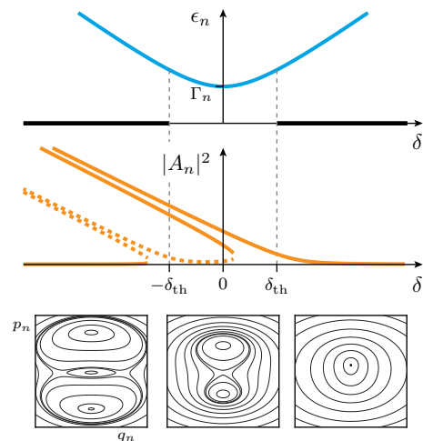
FIG. 13. Degenerate parametric oscillation. Upper panel: blue line indicates threshold of instability, \epsilon_n(\delta) ; bold black line indicate stability region of the ground state. Middle panel: stationary response to applied on-resonance signal vs detuning, intensity of the response indicates the one of the self-sustained oscillations split by the input; solid lines indicate stable solutions born at the edge \delta = \delta_{th} , dashed lines indicate unstable solutions born at the edge \delta = -\delta_{th} . Lower panel: phase portraits of oscillations at different detuning: stable ground state at blue detuning, \delta > \delta_{th} , bistable excited states at -\delta_{th} < \delta < \delta_{th} , and excited states coexisting with the stable ground state at red detuning, \delta < -\delta_{th} .
