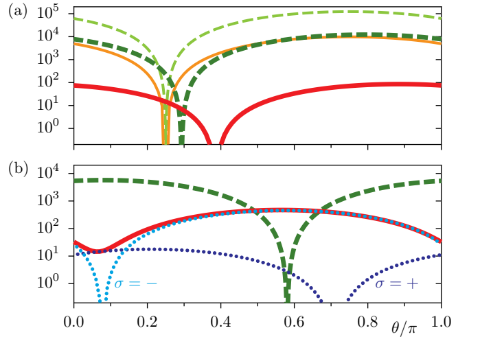
FIG. 25. Squeezing of output quantum noise spectral density and strongly amplified on-resonance signal, (a) for degenerate resonance at \epsilon = 0.95\Gamma , and (b) for non-degenerate resonance at \epsilon = \Gamma 39,46 . Solid red lines refer to quantum noise squeezing spectrum S_n^\theta(0) , bold green dashed lines refer to classical quadrature response \overline{P_0}/|B_n|^2 . In (a) the squeezing directions almost coincide for the signal and noise; thin lines show S_n^\theta(0) (orange solid line) and \overline{P_0}/|B_n|^2 (light green dashed line) in the linear approximation. In (b) blue dotted lines show misoriented supermode contributions to S_n^\theta(0) ; squeezing direction of noise almost coincides with the signal maximum amplification. [ \delta = 0 , |B_n|^2 = 0.1\Gamma , \theta_B = 0 , \Gamma_n = \Gamma_m , \alpha_n = \alpha_m = \Gamma/100 , \Gamma_n = \Gamma_{n0} .]
