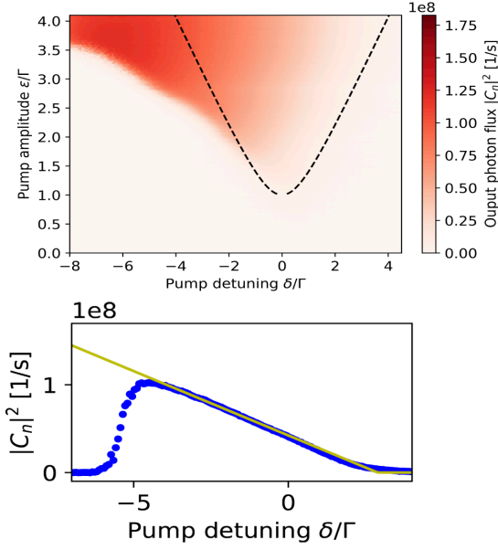
FIG. 14. Experimentally measured intensity of parametric oscillation as function of pump detuning and intensity 67 . Dashed line in upper panel shows instability threshold; oscillation intensity gradually increases at the threshold at \delta > \delta_{th} , and sharply disappears at \delta < -\delta_{th} . Lower panel compares a theoretical prediction 39 (yellow line) and experimental observation (blue dots).
