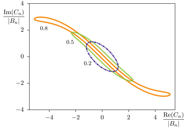
FIG. 7. Anisotropy of the cavity output field in the complex C_n -plane under variation of input phase \theta_B \in [0, 2\pi) , for degenerate parametric amplifier at pump strengths \epsilon_n/\Gamma_n = 0.2, 0.5, 0.8 (purple, green, orange), the purple curve depicts the linear regime, other curves refer to nonlinear amplification discussed in Sec. III C. [ \delta = 0 , \Delta = 0 , |B_n|^2 = 2\Gamma_n , \alpha_n = \Gamma_n/100 .]
