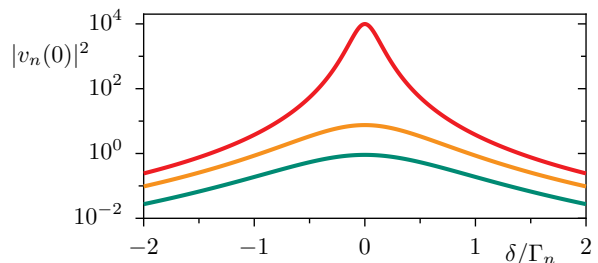
FIG. 6. Linear amplification of undetuned input signal, \Delta = 0 , for degenerate parametric amplifier: idler gain, G^I(0) = |v_n(0)|^2 , vs pump detuning \delta , for increasing pump strengths, \epsilon_n/\Gamma_n = 0.4, 0.7, 0.99 (from bottom to top).
