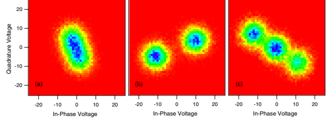
FIG. 15. Experimental histograms of output radiation at different detuning regions 30 corresponding to phase portraits in Fig. 13: (a) squeezed vacuum at \delta > \delta_{th} , (b) two phase degenerate oscillator states at |\delta| < \delta_{th} , and (c) coexisting oscillations and ground state at \delta < -\delta_{th} .
