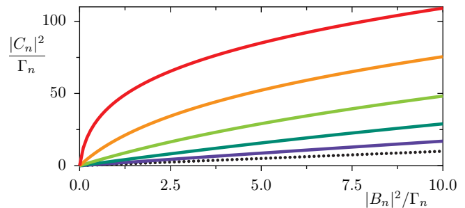
FIG. 9. Output power |C_n|^2 vs input power |B_n|^2 , for the degenerate parametric amplifier with on-resonance input signal, \Delta = 0 , and \epsilon_n/\Gamma_n = 0, 0.2, 0.4, 0.6, 0.8, 1.0 (from bottom to top); the dotted line refers to the Duffing limit \epsilon_n = 0 . ( \delta/\Gamma_n = 0.5 , \theta_B = \pi/2 , \alpha_n/\Gamma_n = 0.01 .)
