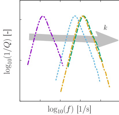
Figure 3.5: Attenuation of a domain containing two perpendicular fractures, for varying permeability of the damage zone k of the control volume given by a mixture rule [56].
