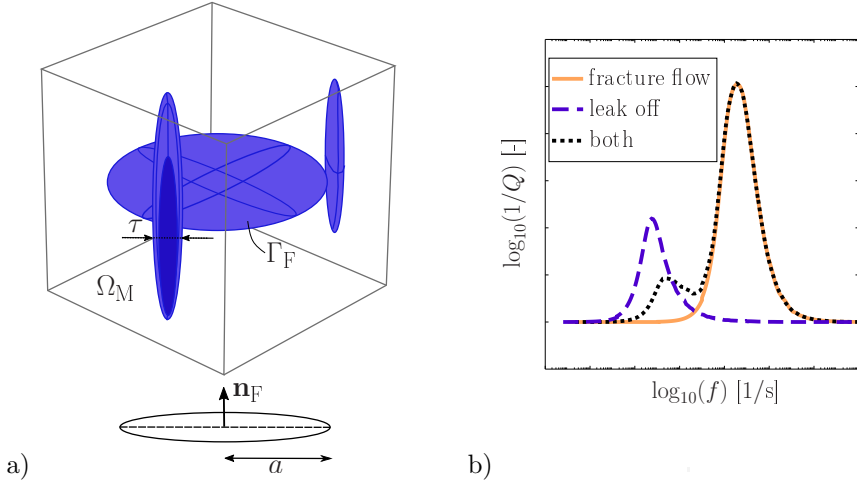
Figure 3.3: Sharp interface model. a) 2-dimensional fractures with fracture aperture \tau(\mathbf{x}, t) in a 3-dimensional domain \Omega_M . b) Fluid-flow mechanisms in between the fractures and from fracture to surrounding matrix.
