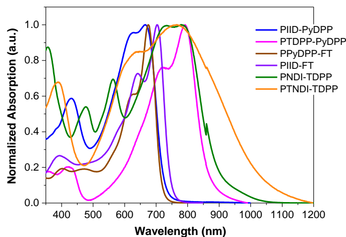
Figure 5.1 Normalized absorption spectra of the polymer thin films
