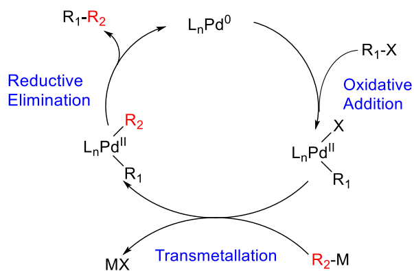
Figure 2.6 Catalytic cycle of the palladium catalyzed Stille and Suzuki reactions
