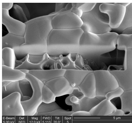
Fig. 6.15 SEM image of a cut performed on the surface of the sample by means of a Focussed Ion Beam.
