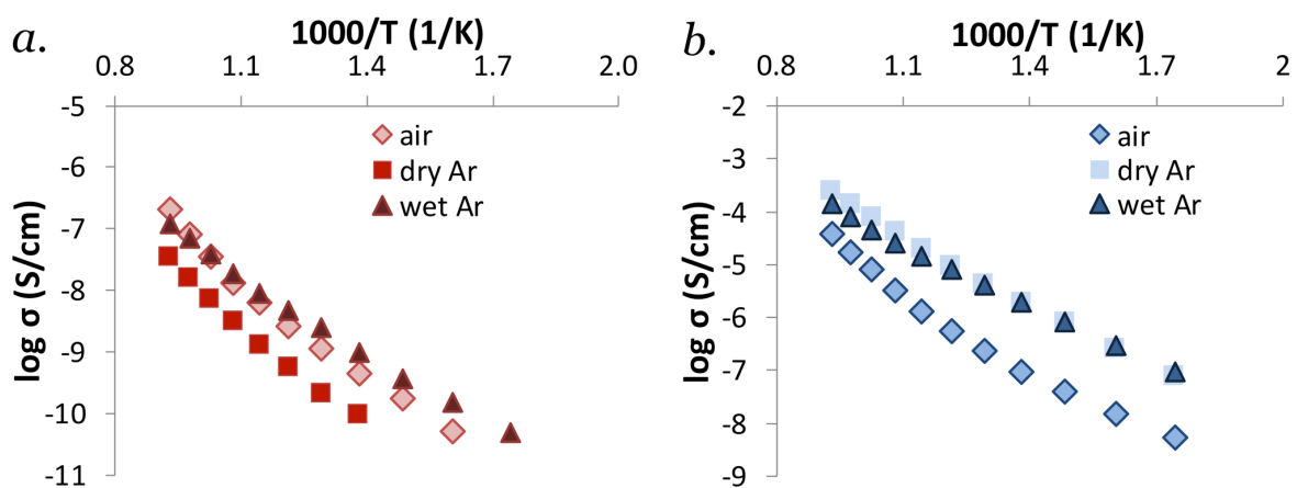
Fig. 6.7 Total conductivity of La_{1-x}Sr_{1+x}ScO_{4-\delta} as a function of inverse temperature, under different conditions. Plot (a.) shows data relative to LaSrScO_4 , while (b.) shows data relative to the doped phase, La_{0.9}Sr_{1.1}ScO_{3.95} .
