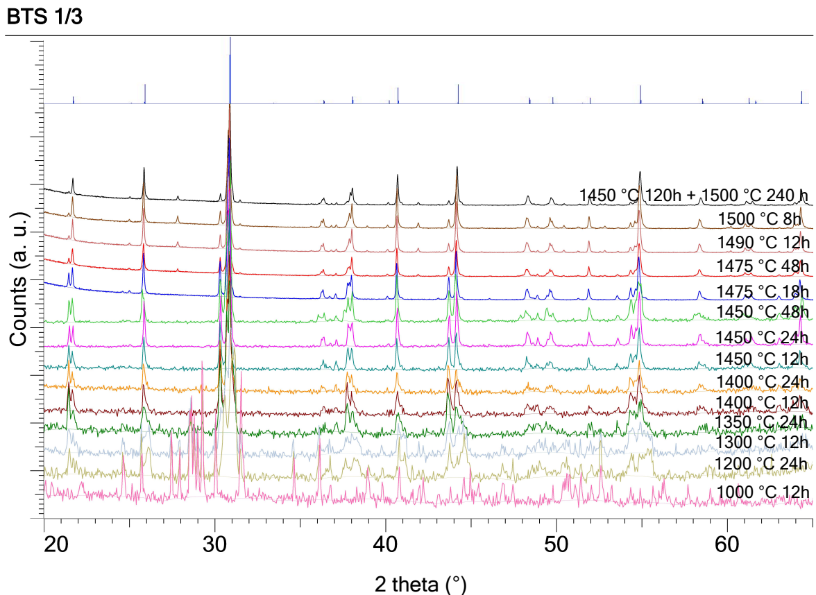
Fig. 5.5 Evolution of the sample BTS_{1/3} with increasing temperature and residence time along the solid-state synthesis steps. The inset on top shows the theoretical Bragg peaks corresponding to a phase of stoichiometry BaTi_{1/2}Sc_{1/2}O_{2.92} built on the basis of the 6H structural model with a = 5.77 \text{ \AA} , and c = 14.14 \text{ \AA} .
