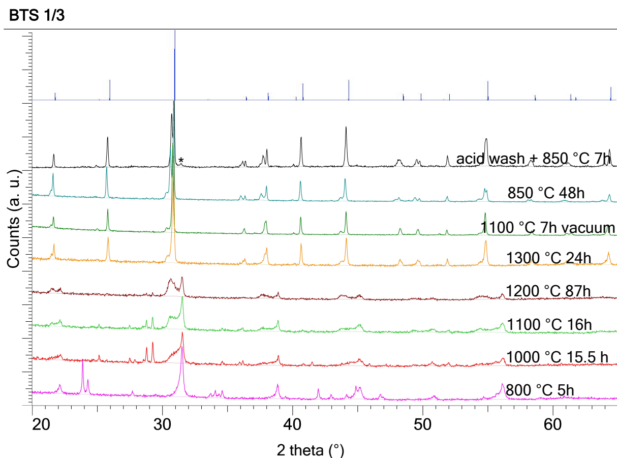
Fig. 5.6 Evolution of the sample BTS_{\frac{1}{3}} produced with the sol-gel method. The asterisk indicates the presence of Sc_2O_3 . The inset on top shows the theoretical Bragg peaks corresponding to a phase of stoichiometry BaTi_{\frac{1}{3}}Sc_{\frac{1}{3}}O_{2.92} built on the basis of the 6H structural model with a = 5.77 Å, and c = 14.14 Å.
