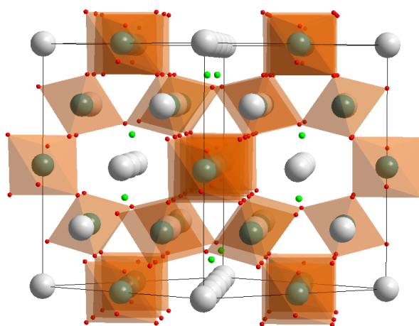
Fig. 3.13 The pyrochlore structure. BO_6 octahedra are highlighted in orange, A-site cations in grey, and non-polyhedral oxygens in bright green. In this representation, the interlinked rings of BO_6 octahedra form channels along the \langle 110 \rangle crystal direction, where the A cations and the non-coordinated oxygens can be found.
