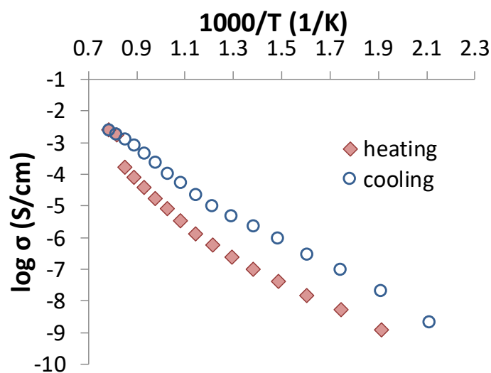
Fig. 6.8 Total conductivity of La_{0.9}Sr_{1.1}ScO_{3.95} as a function of inverse temperature, measured in air, in the temperature range 200 °C to 1000 °C. The two curves show the behaviour during the heating and cooling ramp.
