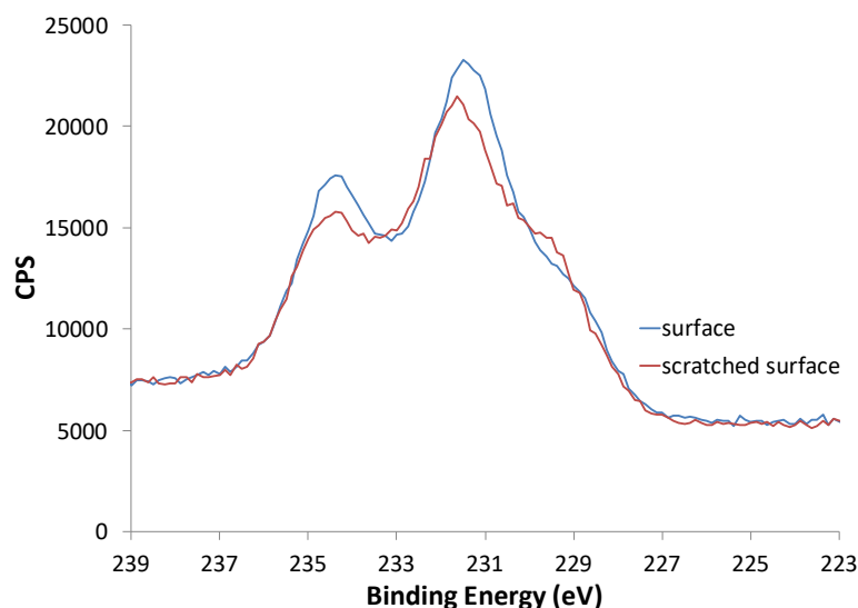
Fig. 6.14 Comparison of the spectral lines of Mo 3d electrons. Spectrum of the surface as-is in blue and spectrum of the abraded surface in red. While the intensity of the peak related to 3d_{5/2} at 231.5 eV decreases, the intensity of the shoulder increases. The observation was related to the increased concentration of Mo^{IV} in the layers immediately under the surface of the synthesised sample.
