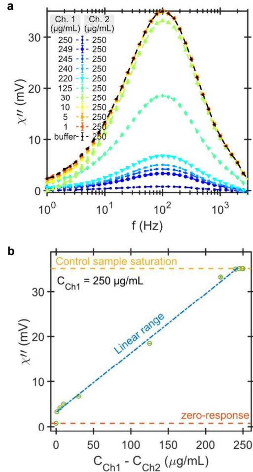
Figure 2 | Calibration of magnetic sensitivity for the differential magnetic readout. (a) Differential measurements of the imaginary component of the magnetic ac susceptibility for several test samples with different concentrations of MNPs ranging from 1 \mu\text{g/mL} to 250 \mu\text{g/mL} in channel 1 with a reference sample in channel 2 containing 250 \mu\text{g/mL} MNPs. Error bars are standard deviation. (b) The amplitude of the imaginary component of the differential ac susceptibility peak at 100 Hz versus the difference in the concentration of magnetic material in the two channels. When the difference in the two concentrations is large (i.e., C_{Ch1} - C_{Ch2} approaches C_{Ch2} ), the background magnetic signal makes it difficult to distinguish small differences in the test sample and the imaginary susceptibility saturates to that of the control sample signal amplitude. The blue line indicates the linear range of the C_{Ch1} - C_{Ch2} (excluding the zero-response and the saturation values) and has a regression co-efficient of 0.99.
