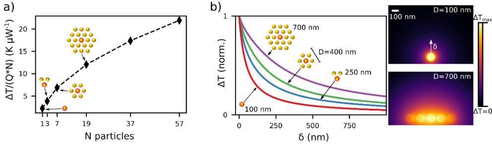
Figure 4 Temperature increase and profile due to collective heating. Temperature increase for collections of gold spheres with 100 nm diameter, and 50 nm edge-to-edge spacing. a) Temperature increase of different collections of uniformly heated gold spheres where the temperature is taken 10 nm from the surface of the central gold sphere (indicated in red), perpendicular to the plane of spheres. Temperature increases are normalized by the total power dissipated by the collection with each individual sphere dissipating the same amount. b) Shown here are the normalized temperature profiles for different planar arrangements of uniformly heated gold spheres. Left: Temperature decay curves extending normally away from the central gold sphere normalized to the maximum temperature in the system. Right: Temperature maps for the smallest planar arrangement (single sphere) and for the largest (19 spheres). Temperature maps are from a plane orthogonal to the plane of the particles.
