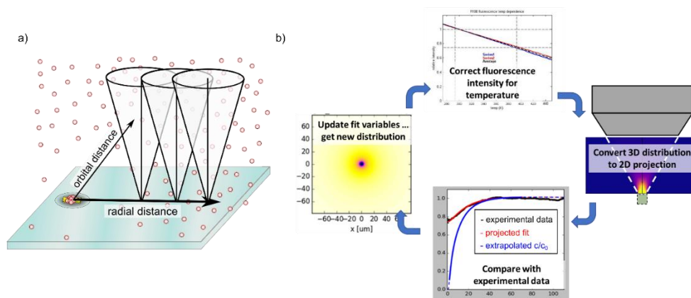
Figure 18 Method of extracting the true thermophoretic depletion via a model-based deconvolution scheme. a) Schematic overview of the procedure. The observed intensity profile is a contribution from all planes of the system containing fluorescent particles based on the collection efficient function of the microscope objective (indicated by the cones). b) Procedure for extracting the true thermophoretic depletion. A 3D concentration profile is assumed for a reasonable value of the Soret coefficient and the depletion is calculated based on the temperature profile. The temperature dependent fluorescence intensity at each point is corrected for. The light collection efficient function is used to determine the corresponding 2D projection of this concentration profile. The 2D projection is then compared with the experimental data. The fitting parameters used are iteratively updated until the calculated projection closely matches the experimental data and the corresponding 3D concentration profile is used for the extracted thermophoretic depletion. Reprinted with permission from 62 . Copyright 2018 American Chemical Society.
