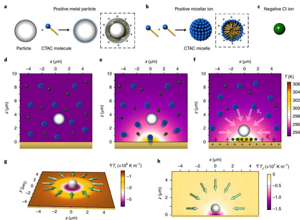
Figure 10 Creating a thermophilic response for a target particle. a) Target particle undergoes surface modification to generate a positive surface charge. b, c) Counterions for the system – b large positive micellar counterions, c small negative Cl counterions. d) Dispersion of target particle and counterions in solution. e) Optical heating creates a temperature gradient, counterions thermophoretically move in response to this gradient. f) Thermophoretically induced counterion concentration gradient creates a standing electric field. This electric field points towards regions of higher temperature causing the positive target molecule to electrophoretically move to the high temperature region. g,h) Simulated temperature gradient and corresponding electrophoretic force direction for in-plane and out-of-plane respectively. Reproduced with permission from 18 . Copyright 2018, Springer Nature.
