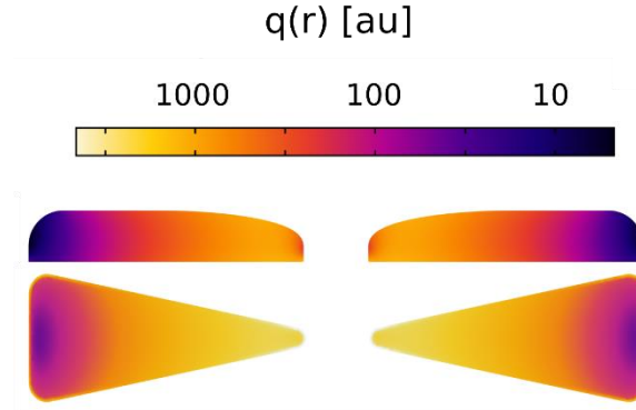
Figure 2 internal heat source density for optically excited plasmonic bowtie antenna. Shown here is the internal heat source density for a gold antenna that is optically excited with linear polarized light, where the electric field points along the long-axis of the antenna.
