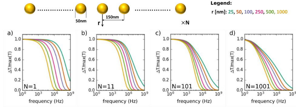
Figure 7 Harmonic heating for linear arrangements of gold particles in water. Extent of temperature modulation for various distances from a line of gold particles vs modulation frequency. a), b), c), and d) correspond to linear arrangements of 1, 11, 101, and 1001 particles respectively with the parameters/spacing shown at the top left. Coloured lines correspond to distances given by legend in top right.
