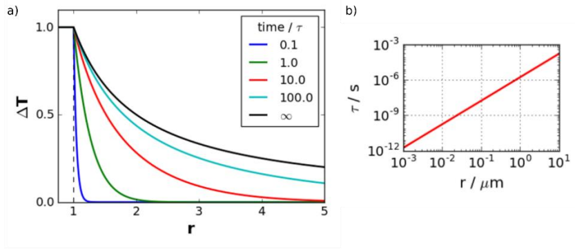
Figure 5 Transient evolution of temperature profile around a single gold sphere. a) Temperature profile after stepwise heating of a gold sphere in water at different times (normalized to time constant at r=a ). Temperature is normalized to the temperature of the sphere and distance is normalized to the radius of the sphere. b) Time constant for temperature evolution in water as a function of distance.
