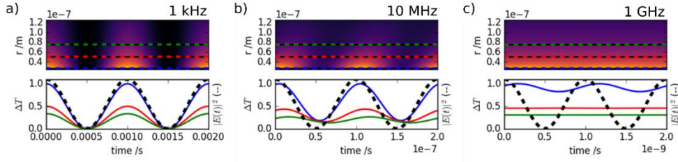
Figure 6 Harmonic heating of a single gold sphere (diameter = 50 nm). Top row: Radial temperature maps vs time at different modulation frequencies. Bottom row: Temperature curves vs time at different modulation frequencies for discrete radial distances. Radial distances correspond to dashed lines in top row. Dashed black line is the heating modulation profile. Modulation frequencies are 1 kHz, 10 MHz, and 1 GHz for a), b), and c) respectively.
