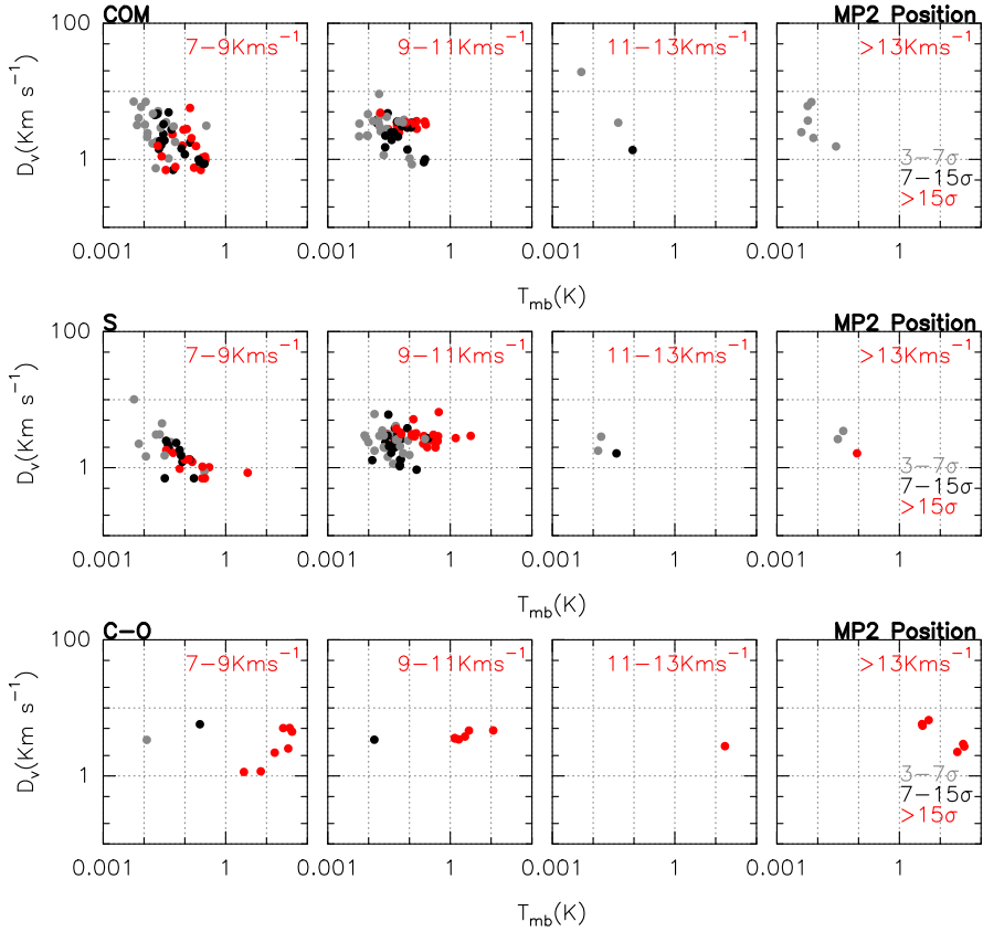
Figure B.59: This figure shows the a comparison between the line width ( D_v ) and the main beam temperature (in K) of the detected lines in the MP2 position. The comparison is done for complex molecules, sulphurated molecules and C-O lines, from top to bottom. The panels are separated in 4 velocity ranges; 7–9 km s -1 , 9–11 km s -1 , 11–13 km s -1 and > 13 km s -1 , from left to right. The gray circle mark the lines with \sigma between 3 and 7, the black circle with \sigma between 7 and 15, and the red ones the lines with \sigma > 15 .
