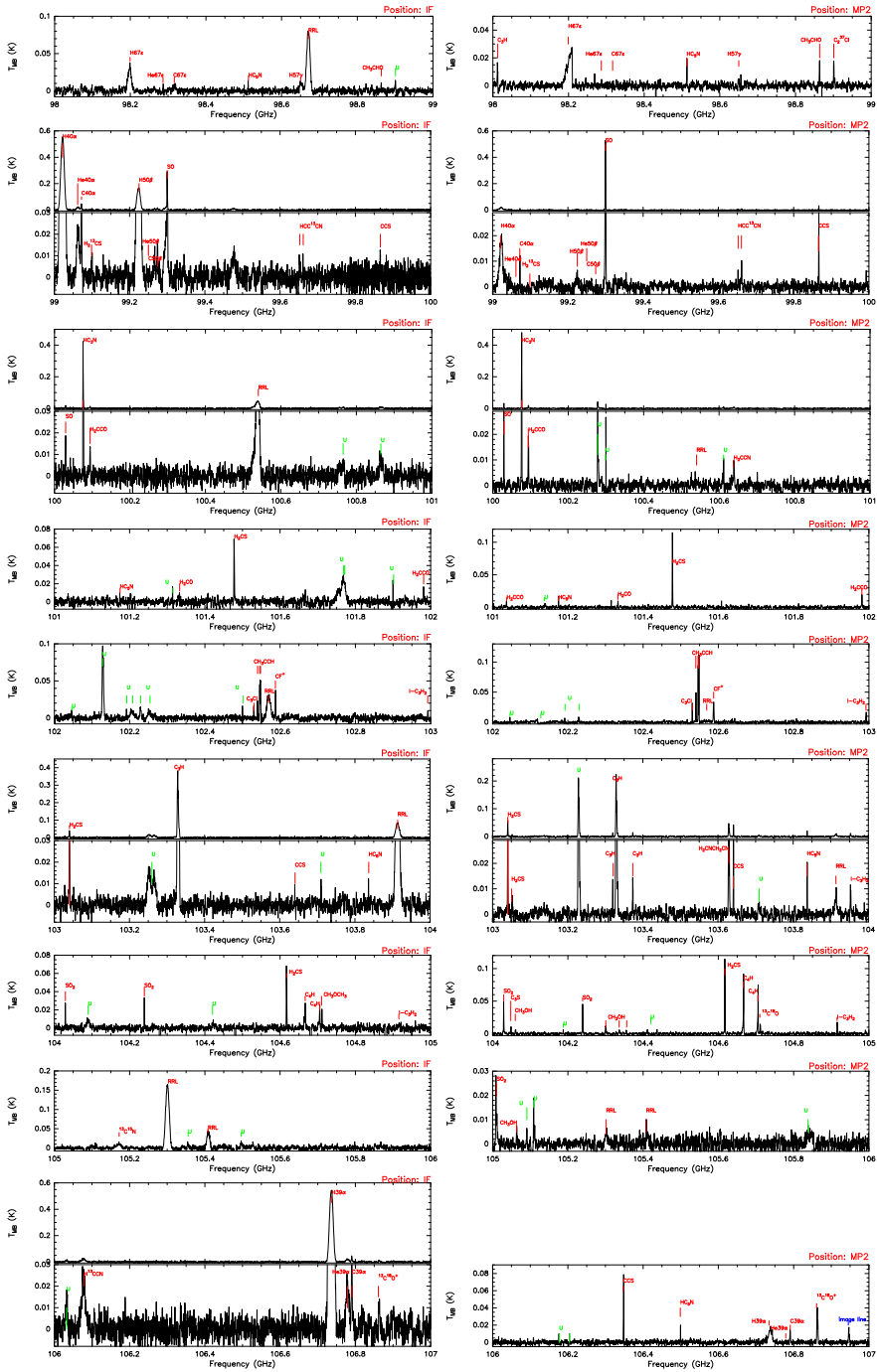
Figure B.3: Spectral survey at 3 mm towards the IF (left) and MP2 (right) position. Continued in next page.
