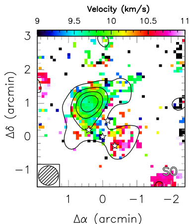
Figure 5.9: Velocity centroid for the SO molecule. The Figure shows the velocity maps over the central observed area (color scale), while black contours indicate SO integrated emission convolved to 30'' . The maps have been produced by computing the first order moment in the velocity range defined in Figure 5.4.
