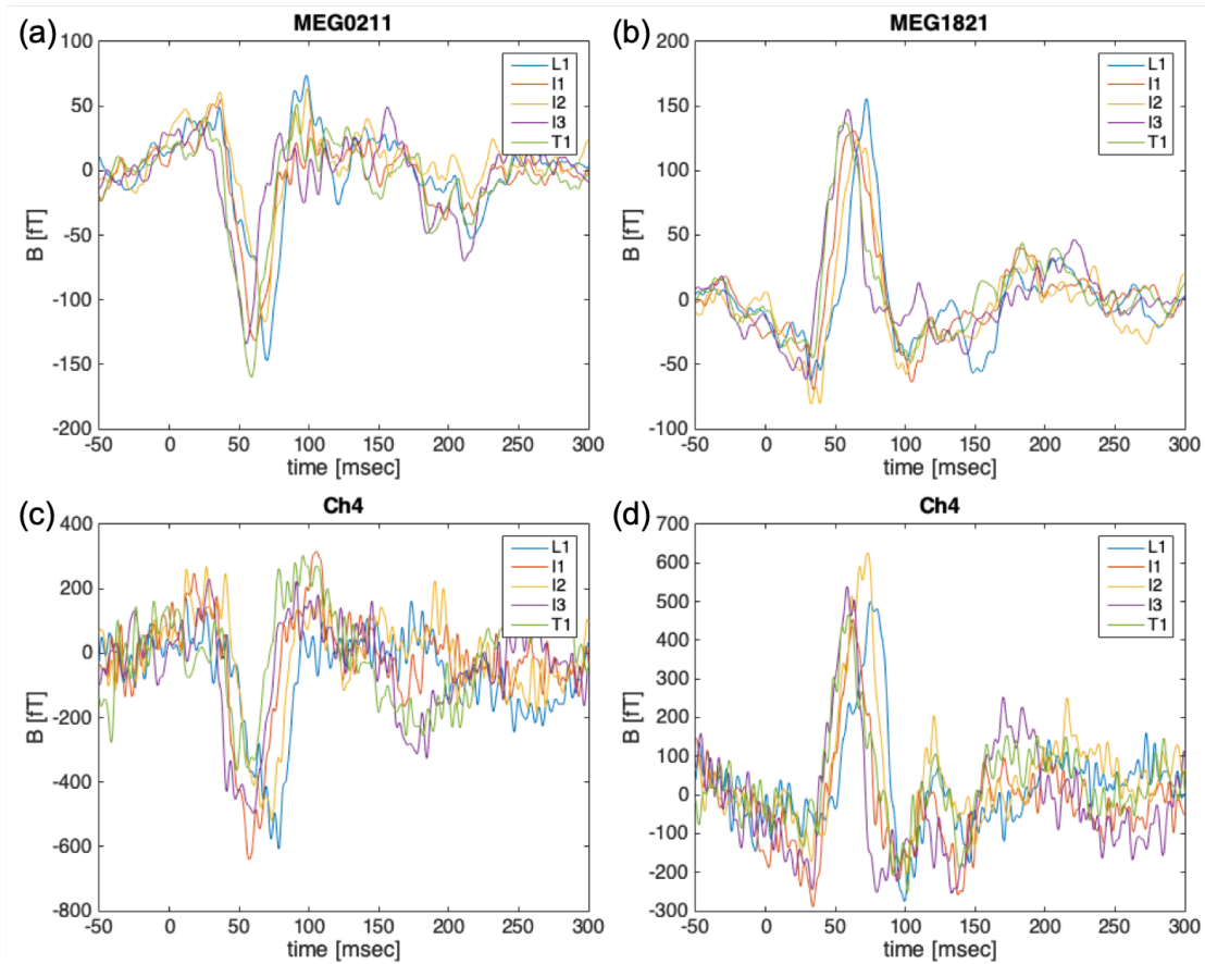
Figure 5.14: Evoked responses to tactile stimulation of different phalanges. a) and b) : Evoked responses recorded with the maximum (negative and positive, respectively) field sensing magnetometers of the TRIUX. c) and d) : Evoked responses for five different phalanges recorded with the central magnetometer of the 7-channel system positioned on the negative and positive, respectively, field maxima.
