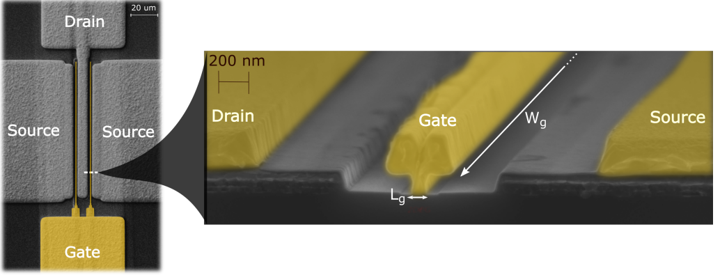
Figure 3.2: Scanning electron microscopy image of a two-finger device and a zoom in on the cross-section of the gate area. Gate area is highlighted in yellow and L_g (100 nm) and W_g (2x100 \mu\text{m} ) are indicated with white arrows.
