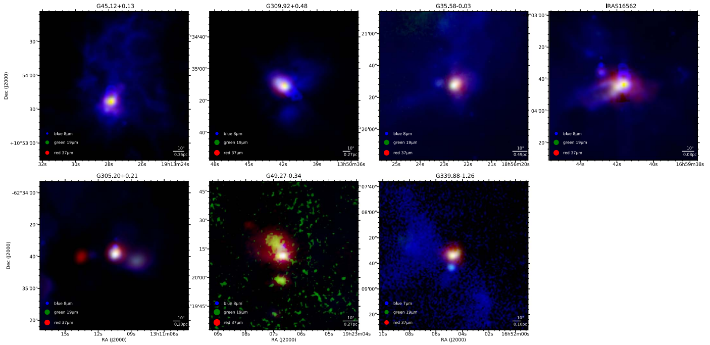
Figure 13. Gallery of RGB images of the seven protostellar sources, as labeled. The color intensity scales are stretched as arcsinh and show a dynamic range of 100 from the peak emission at each wavelength, except for the 19 \mu\text{m} image of G49.27, where only a dynamic range of 10 is shown because of its relatively low signal-to-noise ratio. The legend shows the wavelengths used and the beam sizes at these wavelengths. SOFIA -FORCAST 37 \mu\text{m} is shown in red. SOFIA -FORCAST 19 \mu\text{m} is shown in green. Blue usually shows Spitzer -IRAC 8 \mu\text{m} , except for G339.88–1.26, where it displays SOFIA -FORCAST 7 \mu\text{m} .
