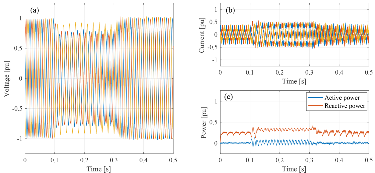
Figure 8. Wind turbine tested for unbalanced voltage dip at low power production: three-phase voltage (a), current (b) and active and reactive power output (c).
