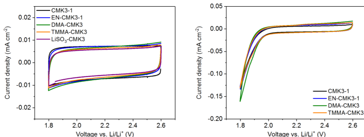
Figure 52. Cyclic voltammograms (CV) for modified CMK3 using two Li-S battery electrolytes. The CV on the right does not contain \text{LiNO}_3 while the one on the left contains 0.4 \text{ M LiNO}_3 .
