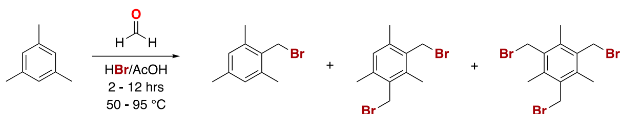
Figure 21. Bromomethylation of mesitylene. 109
