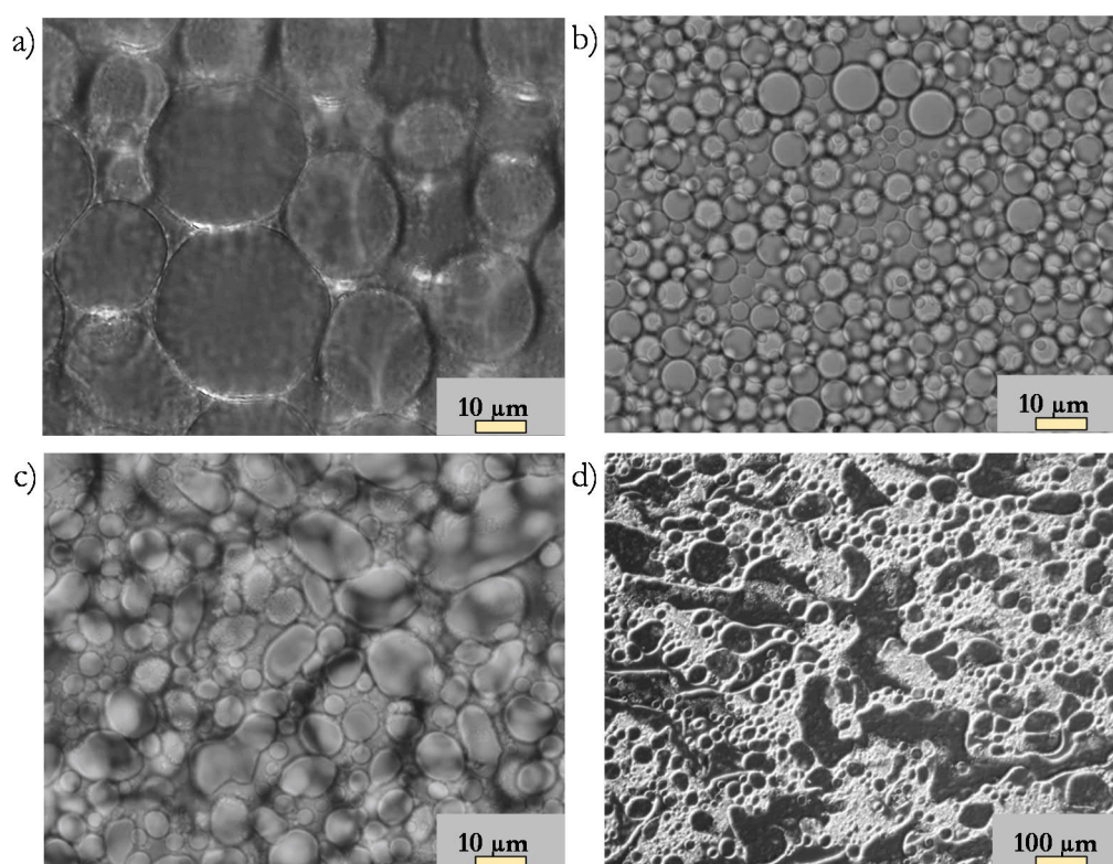
Figure 36. Micrographs of butanol emulsions, stabilized by \text{propyl}_{0.93}/\text{mPEG}_{0.27}\text{-SiNPs} , taken the day of emulsification, after being cooled to room temperature. a) Prepared at 45 °C, with the aqueous phase adjusted to pH 7, at 100 mM \text{CaCl}_2 (expected PIT 71 °C). b) Prepared at 80-90 °C, with the aqueous phase adjusted to pH 7, without added salt (expected PIT 92 °C). c) Prepared at 53 °C, with the aqueous phase adjusted to pH 2, without added salt (expected PIT 48 °C). d) Prepared at 43 – 67 °C, with the aqueous phase adjusted to pH 2, without added salt (expected PIT 48 °C).
