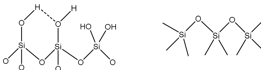
Figure 8. Examples of groups involving Si-O bonds identified on the surface of amorphous silica: vicinal and germinal silanol groups (left) and surface siloxanes (right).
