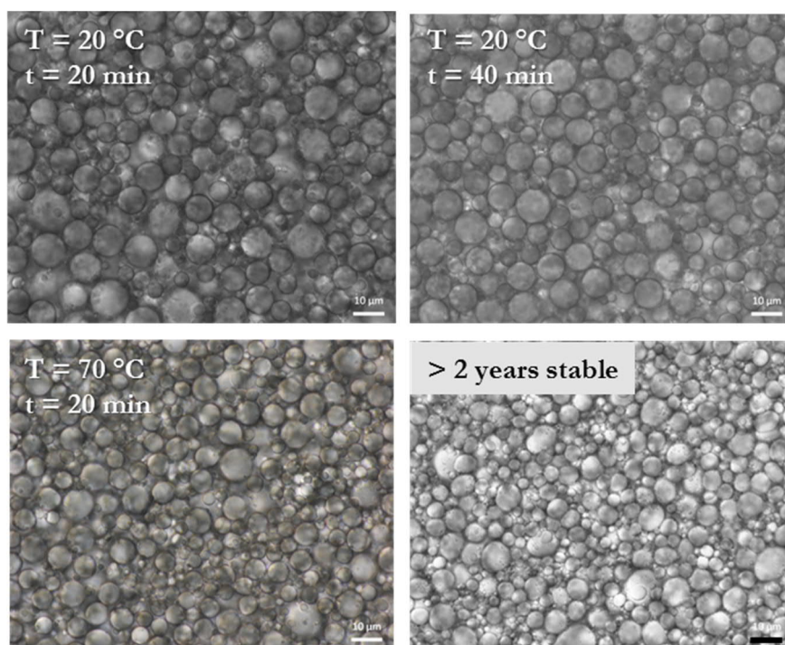
Figure 39. Olive oil emulsions stabilized by propyl 0.93 /mPEG 0.27 -SiNP, with the aqueous phase adjusted to pH 4. Increasing the temperature results in smaller emulsion droplets and an emulsion with very high stability towards coalescence was obtained: almost no change in emulsion droplet size was observed over the course of more than 2 years.
