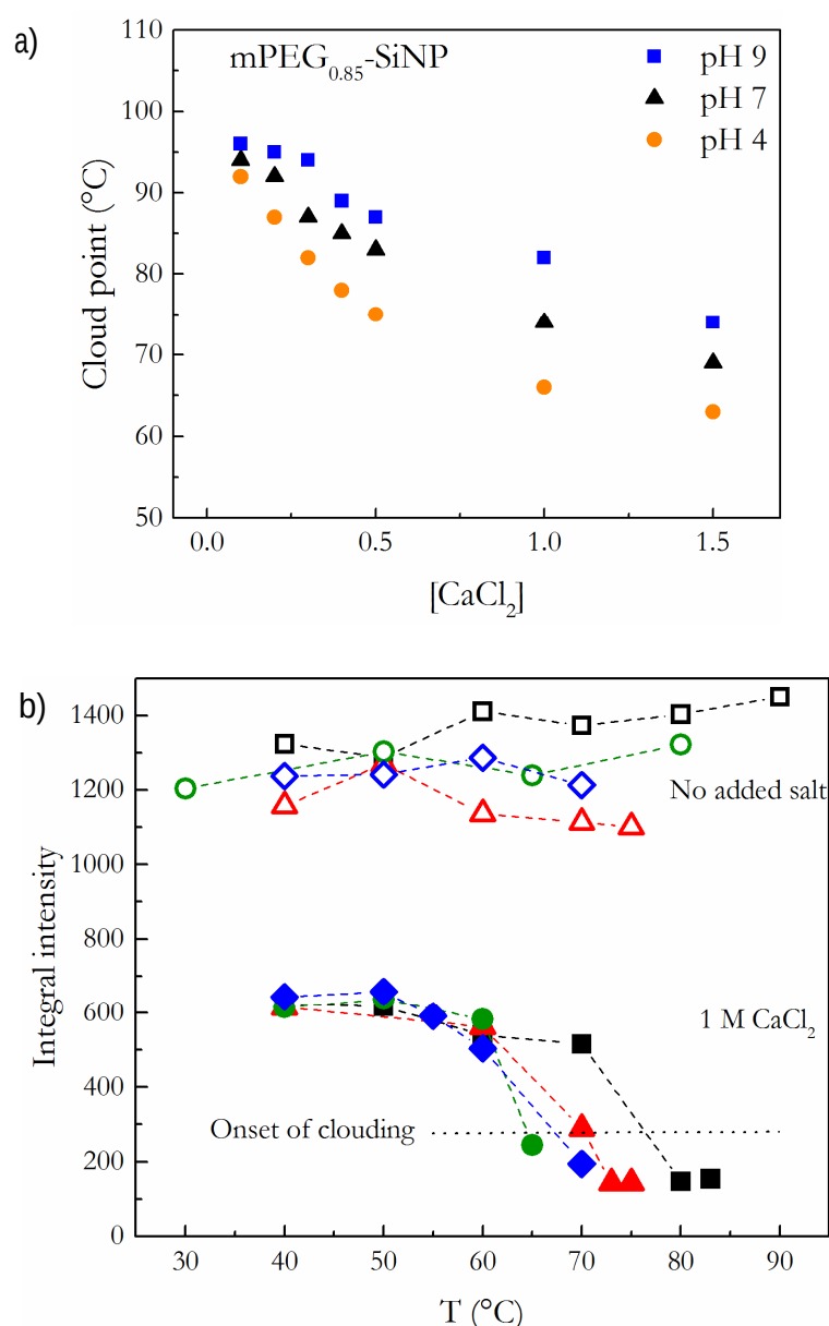
Figure 29. a) Cloud point observed in suspensions with mPEG 0.85 -SiNP 130 , at 2 wt% of SiO 2 , as a function of \text{CaCl}_2 concentration in M, and at varying pH conditions. b) Integral intensities, obtained from ^1\text{H} NMR spectroscopy, of the peak arising from the poly(oxy ethylene) units in the mPEG silane in mPEG 0.85 -SiNP 130 , at 1 M \text{CaCl}_2 and without added salt, at varying pH conditions (pH 9: black ■/□; pH 7 red ▲/△; pH 4 green ●/○; pH 2 blue ◆/◇). Reprinted from Paper II.
