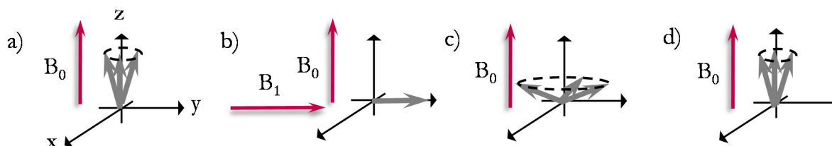
Figure 15. Using the descriptive vector model, showing magnetization from magnetic moments of the nuclear spins in a sample: a) The magnetic moments align with the applied magnetic field B_0 and precess about the z-axis with net magnetization along the z-direction; b) An RF pulse has been applied, creating the magnetic field B_1 , the magnetic moments align coherently in the xy-plane; c) Relaxation in both the z-direction and the xy-plane; d) Back at thermal equilibrium.
