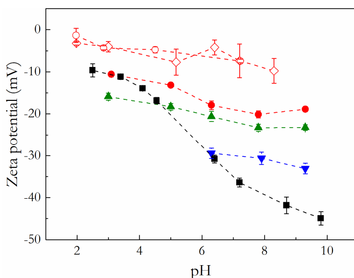
Figure 22. Zeta potential of dialyzed PEGylated samples as a function of pH, with varying salt concentrations and surface coverages: samples with 0.068 (blue ▼), 0.155 (green ▲) and 0.315 (red ●) μmol mPEG silane m -2 are measured at 7 mM salt. Unmodified particles (black ■) are shown for comparison and have ~10 mM salt. For high surface coverage it was possible to measure at higher salt concentrations; 100 mM (red ○) and 200 mM (red ◇). Reprinted from Paper I ©2015 with permission from Elsevier.
