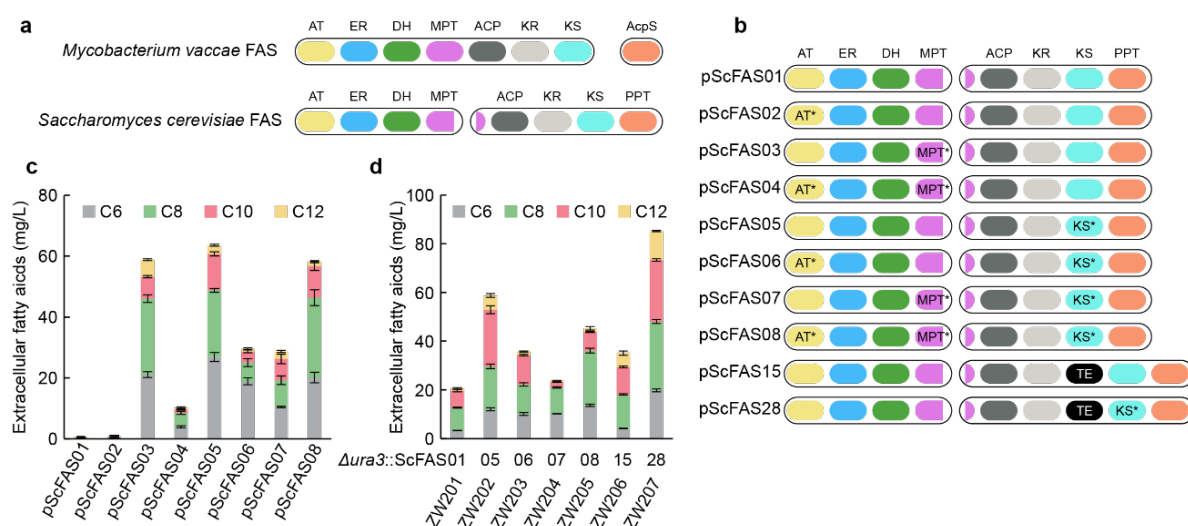
Figure 22. The synthesis of MCFAs in strains with engineered fFASI enzymes. (a) Overview of domain composition of the FASI enzymes from S. cerevisiae and M. vaccae . (b) Schematic overview of engineered fFASI. (c) The production of extracellular MCFAs by strains containing plasmids encoding engineered fFASI. (d) The production of extracellular MCFAs by strains with engineered fFASI genes integrated. Adapted from Paper III.
