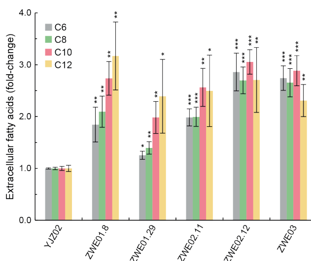
Figure 30. The synthesis of MCFA from evolved strains compared to those from parental strain YJZ02.
