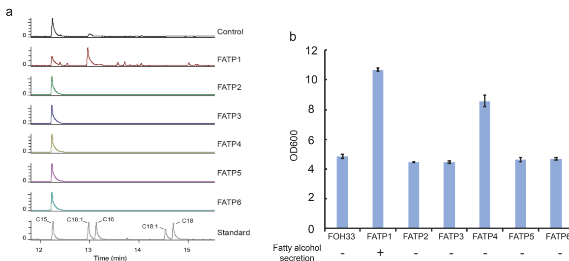
Figure 6. The effect of expression of FATP family transporters in a high fatty alcohol production yeast strain, FOH33. (a) GC spectra of strains based on FOH33 containing FATP transporter isoforms. FOH33 carrying the empty vector pLYH01 was used as control. (b) The final biomass (represented as OD600) of FOH33-derived strains expressing FATP proteins or carrying an empty vector. Increased production of extracellular fatty alcohols (+) or no effect (-) compared to control strain is indicated according to (a). Adapted from Hu et al. 84
