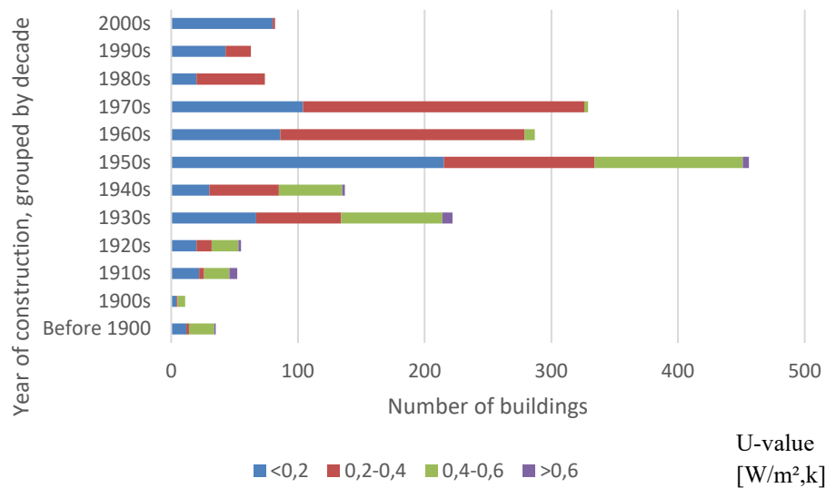
Figure 6 - Distribution of U-value of roofs for buildings in the municipal housing stock grouped by year of construction.
