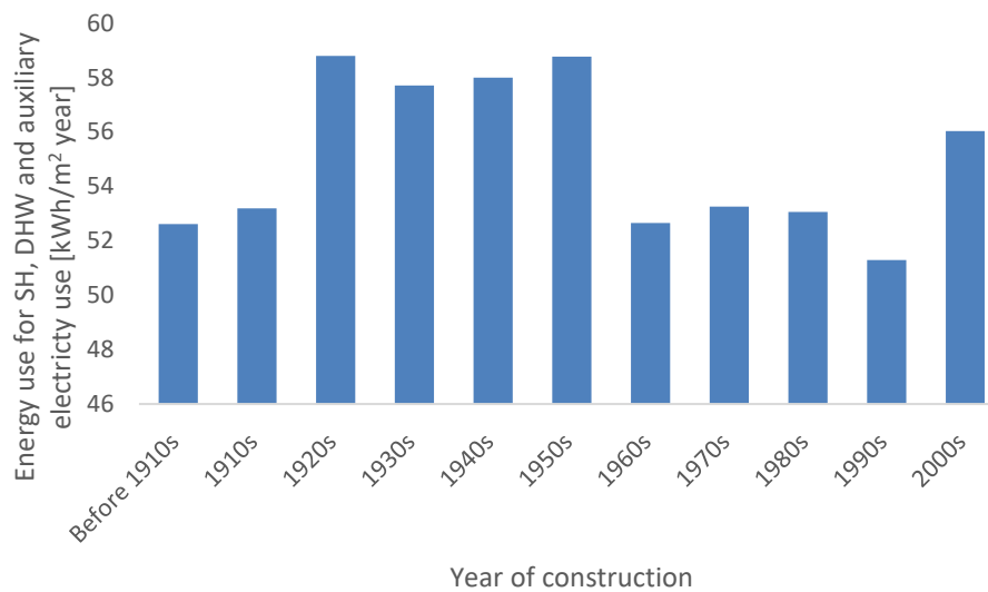
Figure 13 – Average final energy use grouped by year of construction for the stock of the municipal housing company after deep renovation.
