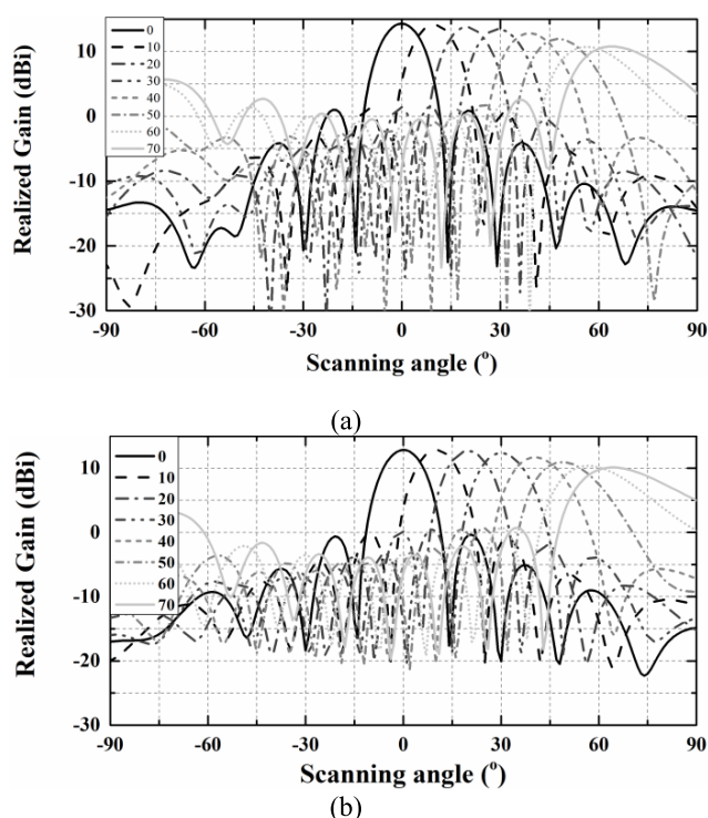
FIGURE 10. Realized beamforming gain of subarrays of (a) endfire polarization and (b) new design.
