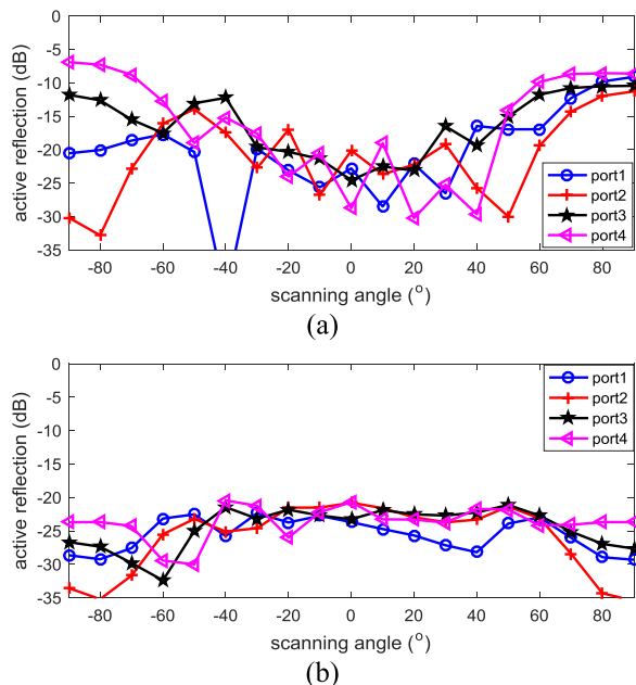
FIGURE 9. Active reflections at ports 1-4 of one subarray of (a) endfire polarization and (b) new design.
