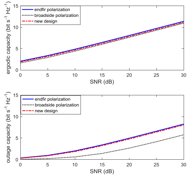
FIGURE 11. Comparisons of ergodic capacities and outage capacities (at 0.01 outage probability) of the three handset arrays.
