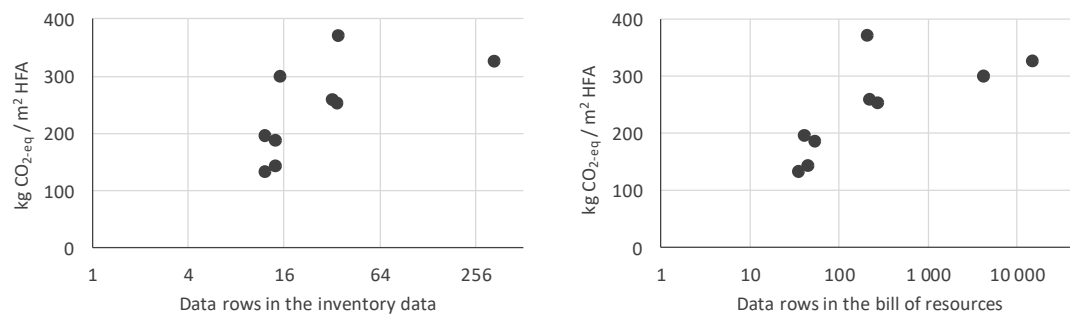
Figure 9: Plotting of LCA results in relation to study specific indicators of data quality expressed in number of data rows in inventory emission data and the inventory bill of resources
