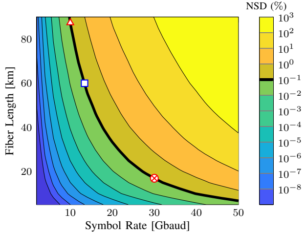
Figure 2: NSD for RP on \beta_2 at different symbol rates and fiber lengths. We considered a QPSK signal with 5 dBm input power.
