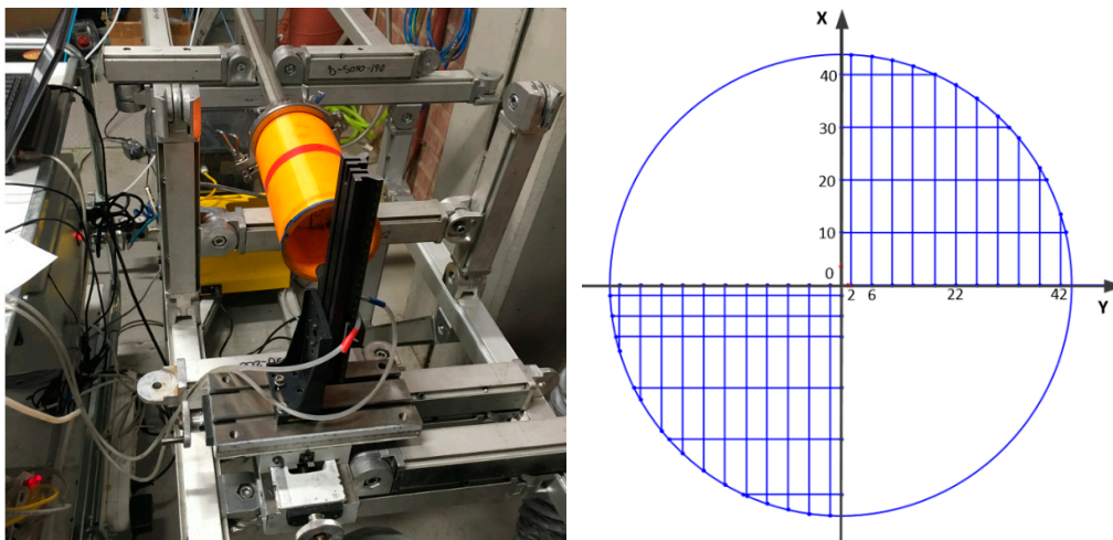
Figure 6. Prandtl sampling setup and sampling position schematic (right).
