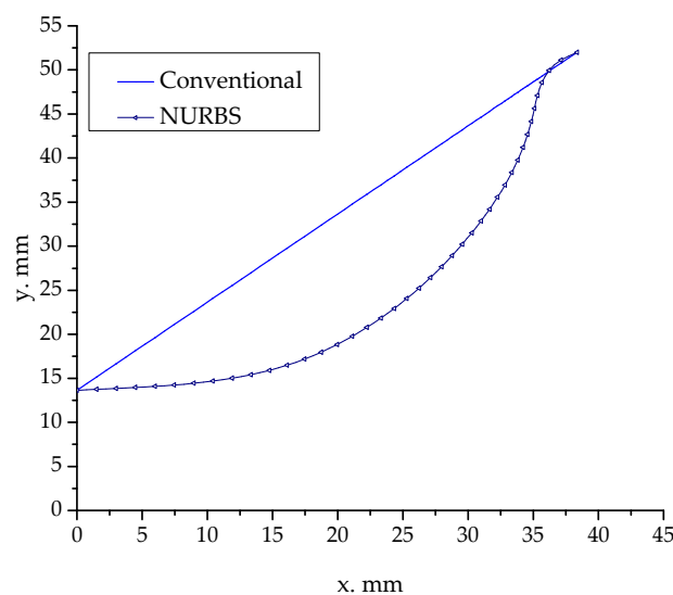
Figure 3. The shapes of the conventional cone and the nonuniform rational B-splines (NURBSs) cone.
