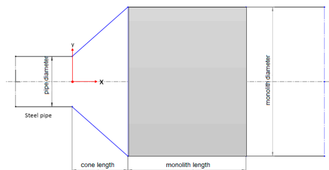
Figure 2. Schematic of the gasoline particulate filter (GPF).
