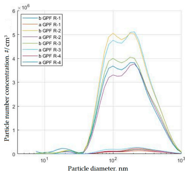
Figure 15. Particle number size distribution for case 1, loading #4. b—before; a—after; R—round.
