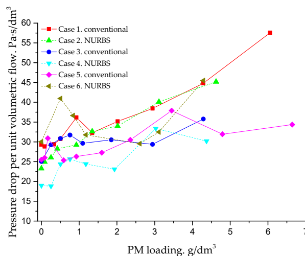
Figure 9. Comparison of the pressure drop per unit volumetric flow.
