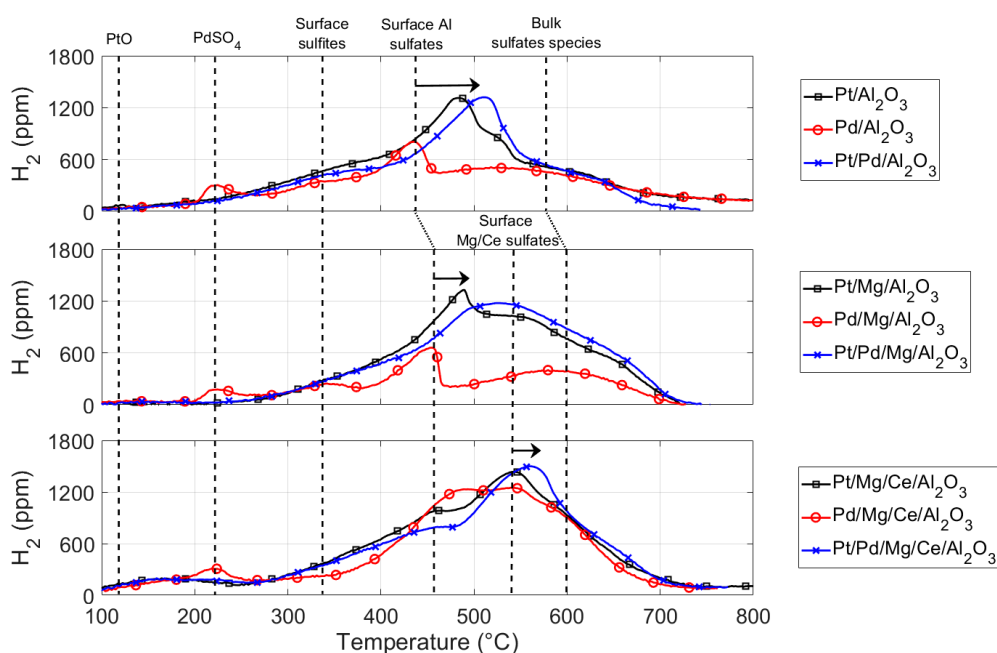
Figure 8. H 2 consumption for all samples during H 2 -TPR experiment in a flow of 1600 ppm of H 2 with a ramp rate of 5 °C/min.
