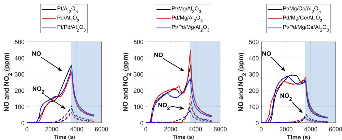
Figure 1. NO and NO 2 profiles over the NO 2 adsorption and Ar flushing (light blue) steps.
