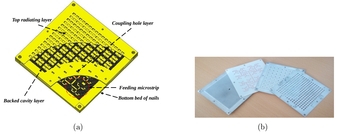
Figure 9: (a) Numerical model of the proposed array antenna in CST Microwave studio . In order to observe the microstrip and waveguide open details the substrate is hidden. (b) Photograph of the proposed 16 \times 16 array antenna fabricated by EDM technology.
