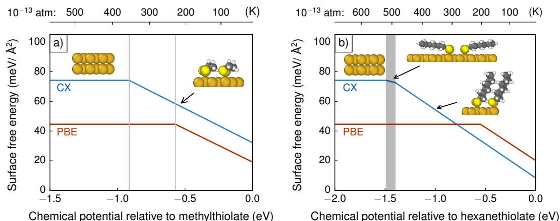
Figure 5.1: Phase stability curves for adsorption of gas-phase alkanethiolates on gold as a function of either the relative chemical potential of the adsorbates or, assuming ultra high vacuum conditions, the temperature. a) For methylthiolates only the clean surface and a dense monolayer are stable. b) For hexanethiolates an intermediate phase is also found where the alkyl chains are almost perpendicular to the surface due to dispersive interactions.
