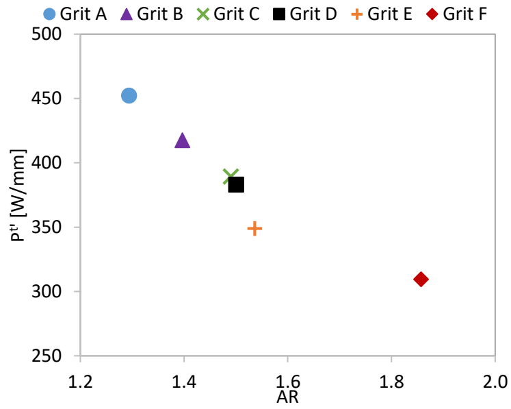
Figure 25: Correlation between power and aspect ratio of grit.
