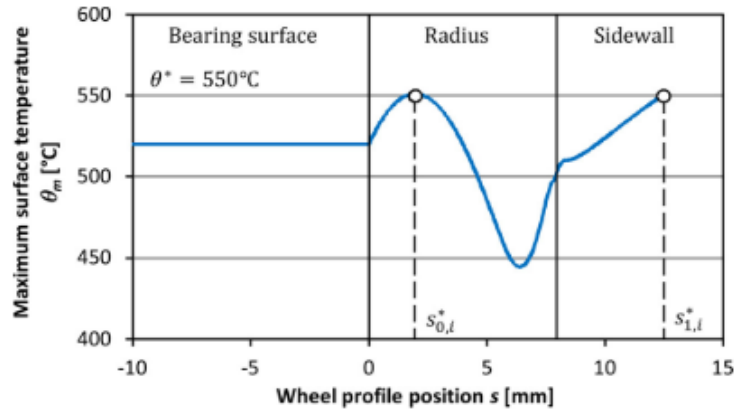
Figure 9: Maximum surface temperature along the wheel profile (Reprinted from Journal of Materials Processing Technology, 259, Radovan Drazumeric, Roope Roininen, Jeffrey Badger, Peter Krajnik, Temperature-based method for determination of feed increments in crankshaft grinding, 228-234, Copyright (2018), with permission from Elsevier)
