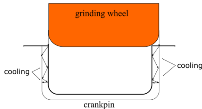
Figure 5: Alternative approach to grinding a crankshaft proposed by JTEKT (Adapted and modified from [9]).
