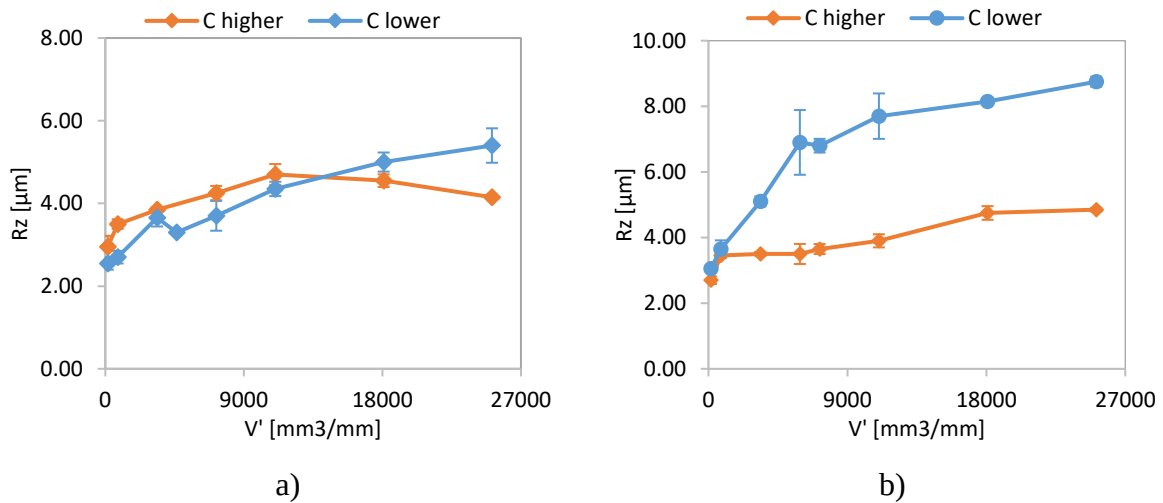
Figure 32: Surface roughness when grinding with a) Parameters A and b) Parameters B.
