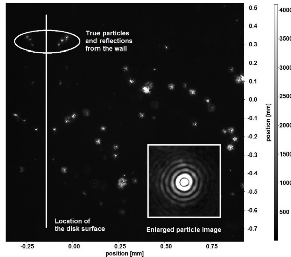
Figure 3: Example of images of registered light scattering signal from the particles and their reflections by the wall
