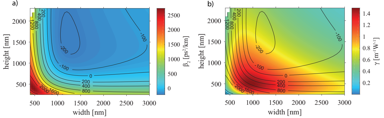
Fig. 8. Waveguide dispersion engineering (a) and the corresponding nonlinear Kerr parameter (b) for a rectangular waveguide with silicon nitride core. According to Fig. 6, this implies that the optimal narrower combs are unattainable for solitons. The right figure shows that the nonlinearities are satisfactory ( \gamma \approx 1 \text{ W}^{-1}\text{m}^{-1} ) for most GVD values, and they can be maximized through suitable design of the cross-section geometry.
