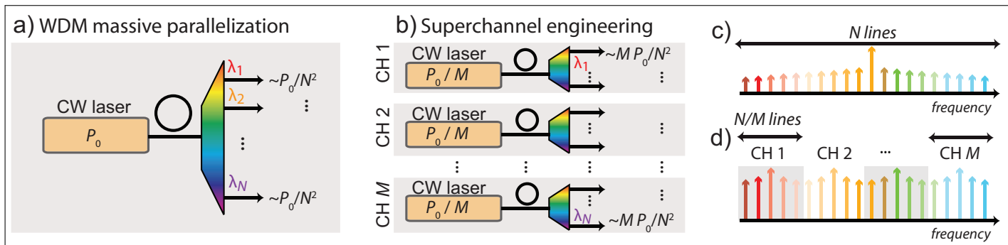
Fig. 1. The diagram in a) shows a basic layout where a single microcomb source provides all lines for a WDM system. In comparison, the diagram in b) shows how the same number of lines can be provided using narrower microcombs in an arrangement of M superchannels. The sketches in c) and d) show the combined comb spectra of the systems in a) and b) respectively before equalization of line power. The system in b) is expected to have M times higher power per line than the system in a), while still using the same total optical input power.
