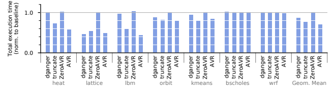
Figure 9: Execution time.
