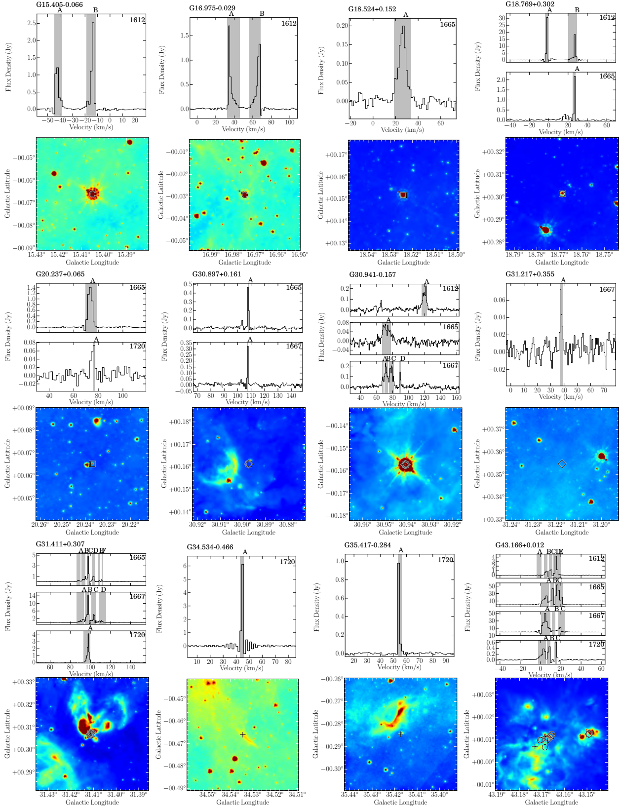
Fig. 2. Examples of individual OH spectra and 8\ \mu\text{m} images for different OH maser lines (remaining maser sites are presented in the Appendix A). For each maser site, the top panels show the spectrum/spectra identified in this region, and the bottom panels present the corresponding GLIMPSE 8\ \mu\text{m} image (Benjamin et al. 2003; Churchwell et al. 2009). Where GLIMPSE data are not available, the corresponding WISE data (Wright et al. 2010) are used. The grey-shaded parts in the spectra outline the velocity regimes of the individual maser spots, and the circles, squares, diamonds, and plus-signs mark the positions of the 1612, 1665, 1667, and 1720 MHz maser spots, respectively (spatially overlapping ones are sometimes difficult to visually separate).
