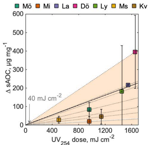
Figure 16. The impact of UV 254 irradiation on AOC produced per unit of DOC ( \Delta\text{sAOC} = \text{AOC}/\text{DOC} ). Solid line: the general linear fit between UV dose and \Delta\text{sAOC} of seven sampling sites. Dashed lines: individual linear fit between each data point and the origin. Impact of UV irradiation on the DBPs.
