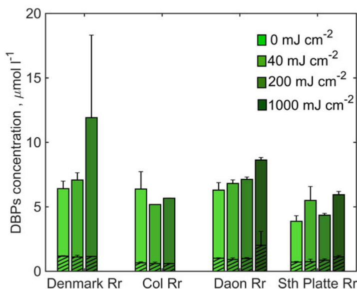
Figure 17. Concentration of disinfection by-products in four chlorinated waters preceded by different UV dose irradiation. Green bars: AOC1 concentration; Hatched area: THM4+HAN6.
