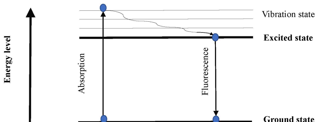
Figure 2. Simplified Jablonski diagram describing the fluorescence phenomenon.
