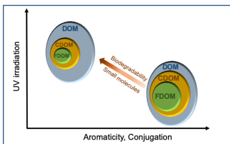
Figure 5. The schematic alteration of the dissolved organic matter (DOM), chromophoric dissolved organic matter (CDOM) and fluorescence dissolved organic matter (FDOM). Upon UV irradiation the FDOM reduces more than CDOM followed by DOM. Overall, the degree of aromaticity, conjugation, molecular size decrease, and biodegradability increase.
