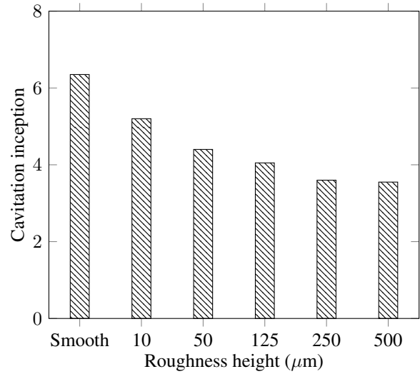
Figure 4: Variation of the cavitation inception versus the surface roughness height for the fully rough foil.
