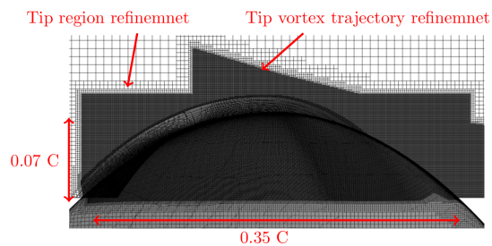
(a) Resolution around the tip, zoomed view
