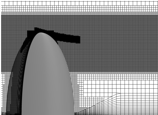
(b) Streamwise mesh distribution
