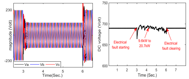
Fig. 3 Waveforms of synthetic voltage dip (left-side) and the regulated DC-link voltage, V_{dc} (right-side).
