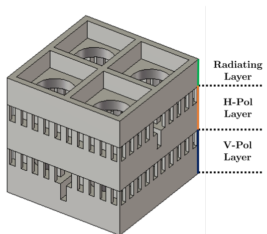
Fig. 5: 2 \times 2 dual-polarized unit cell.
